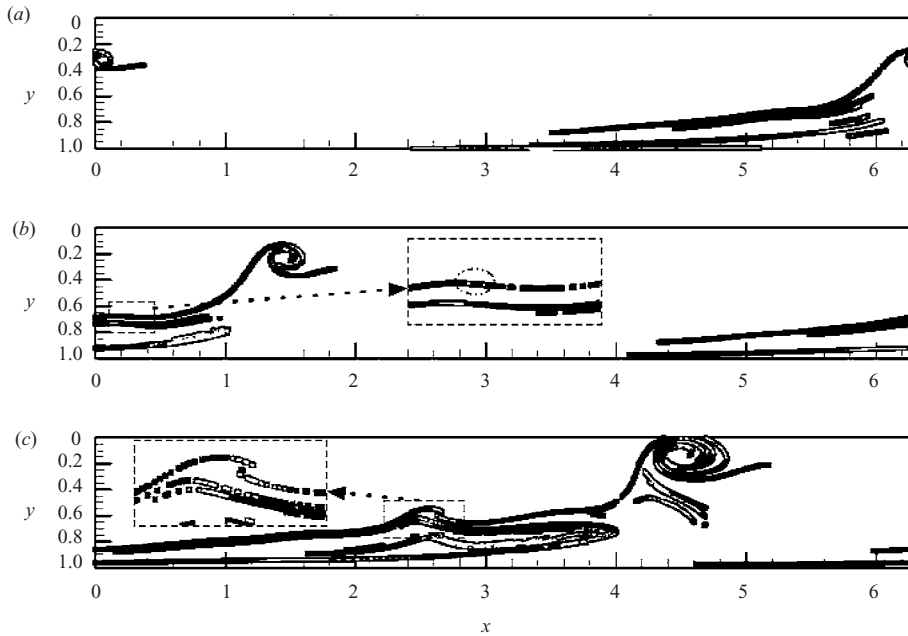
FIGURE 6. Magnitude of \langle \mathbf{n}, \mathbf{Sn} \rangle along spanwise-constant cross-sections of LCS surfaces at times (a) t^+ = 45 , (b) t^+ = 63 , and (c) t^+ = 99 . Negative strain rate (compression normal to the surface) is black; positive strain rate (expansion) is white with black outline.
