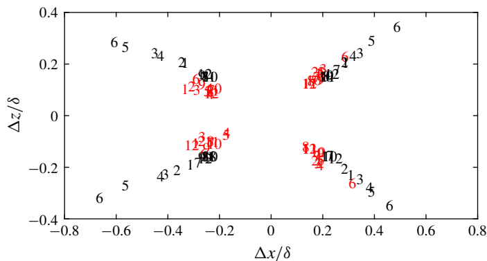
FIGURE 34. Location of peak magnitude of R_{uw} in each quadrant of x - z plane for case 2. Numbers plotted indicate streamwise station number. Red indicates y/\delta = 0.15 , black y/\delta = 0.4 .
