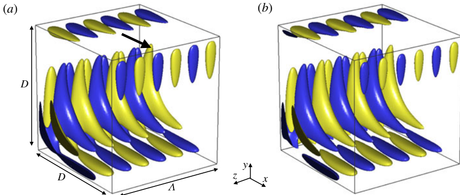
FIGURE 1. Representation of TGL vortices in the lid-driven cavity flow at Re = 1200 and \Lambda/D = 0.945 ; lid moves in the direction of arrow. Snapshot of isosurfaces of 20% max/min spanwise velocity of spanwise Fourier mode \beta = 3 . (a) DNS, (b) resolvent-based model. Animations of isosurfaces of DNS and model are shown in supplementary movies 1 and 2 respectively, available at http://dx.doi.org/10.1017/jfm.2016.339 .
