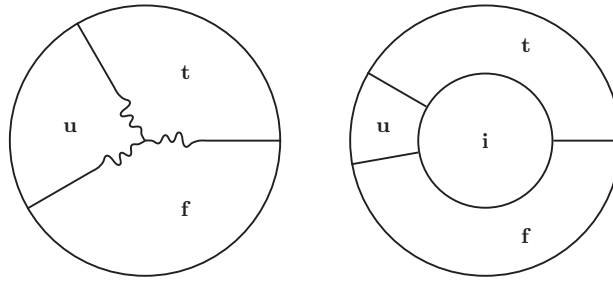
Fig. 4. Least versus typical intended \sqsupseteq^4 -model.
