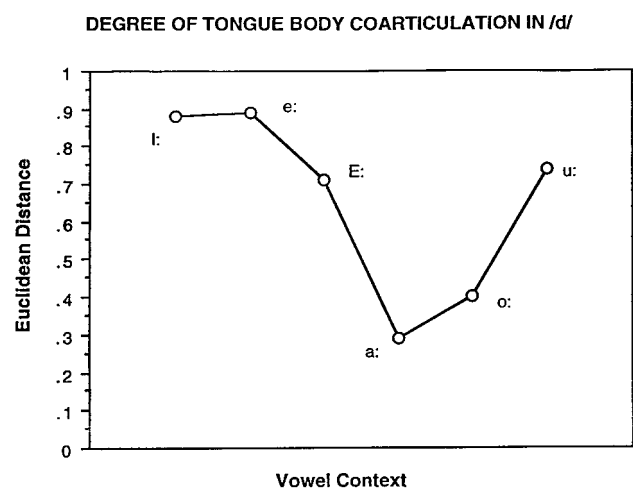
Figure R1. Degree of tongue body coarticulation measured in Euclidean distance for six Swedish vowels in the context of a retroflex [d]. Values were obtained from apex model simulations.
