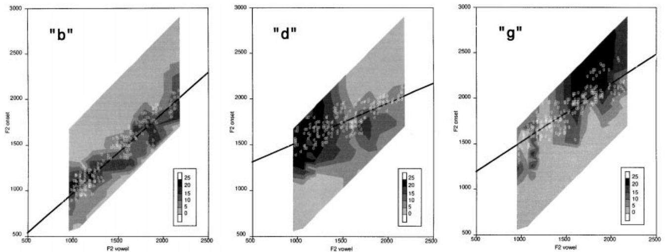
Figure 15. Identification surfaces for “b,” “d,” and “g” showing correspondences between perceptual results (gray scales) and acoustic speech data (white “b-d-g” letter overlays) in locus equation space. Darkest regions reflect unequivocal identification of a consonant in response to synthesized CV stimuli varying across a full range of F2 onsets for each of 10 vowels.
