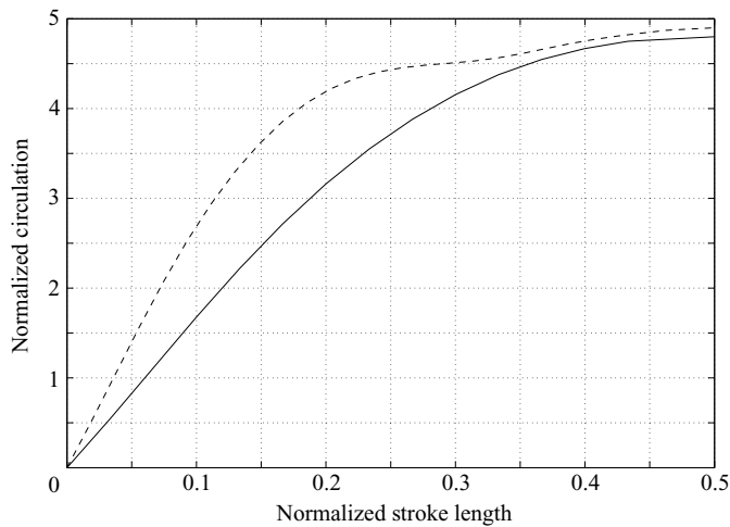
FIGURE 6. Normalized circulation of the leading-edge vortex estimated from DPIV measurements, for an optimal half-stroke (continuous line) and a suboptimal one which is 20% longer (dashed line). Abscissas are normalized with the length of the full stroke.
