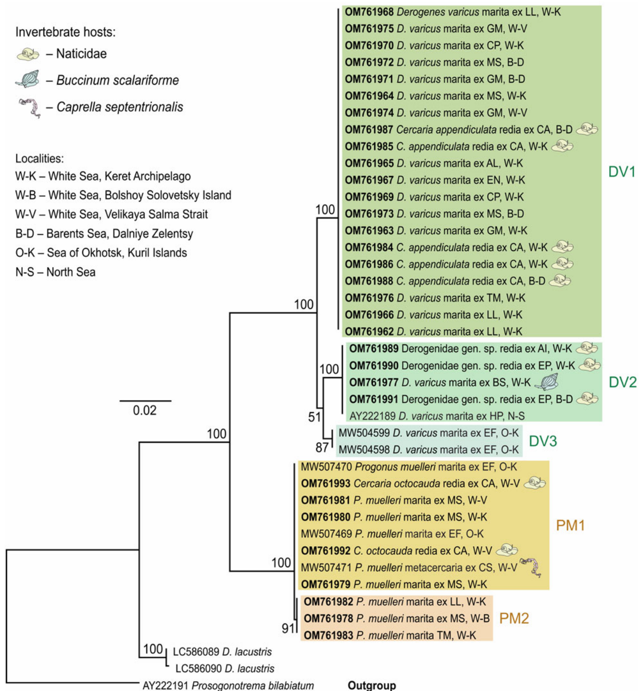
Fig. 1. ML phylogenetic tree based on the 28S rDNA sequence data. Bootstrap values are printed in nodes. Scale bar shows the substitution rate. DV1–3 and PM1–2 mark the separate genetic lineages within Derogenes varicus and Progonus muelleri species, respectively. Abbreviations: AI – Amauropsis islandica ; AL – Anarhichas lupus ; BS – Buccinum scalariforme ; CA – Cryptonatica affinis ; CS – Caprella septentrionalis ; CP – Clupea pallasii marisalbi ; EF – Eumicrotremus fedorovi ; EN – Eleginus nawaga ; EP – Euspira pallida ; GM – Gadus morhua ; HP – Hippoglossoides platessoides ; LL – Limanda limanda ; MS – Myoxocephalus scorpius ; TM – Triglops murrayi .
