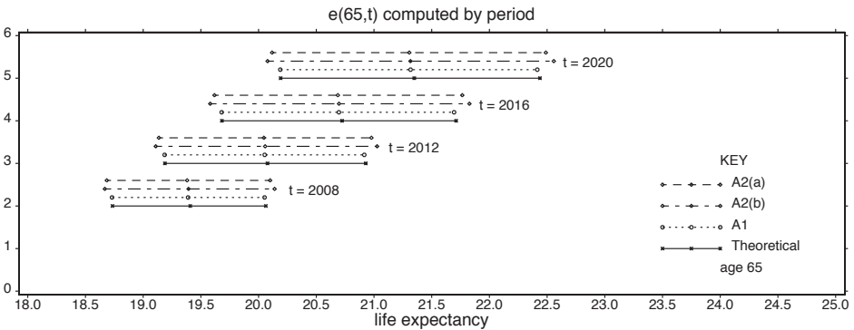
FIGURE 2A: (b) computations by period, age 65, various periods (t > 2004).
