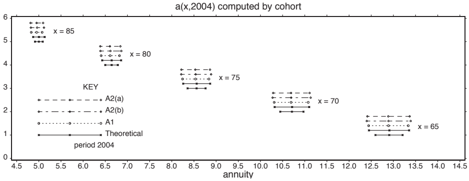
FIGURE 2B: (a) computations by cohort, period 2004, various ages (x).
