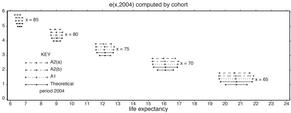
FIGURE 2A: (a) computations by cohort, period 2004, various ages (x).
