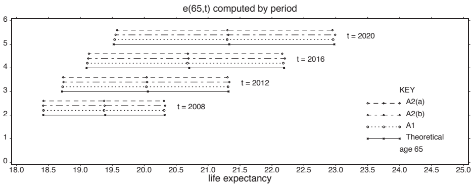
FIGURE 3A: (b) computations by period, age 65, various periods ( t > 2004 ).
