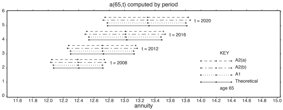
FIGURE 2B: (b) computations by period, age 65, various periods (t > 2004).
