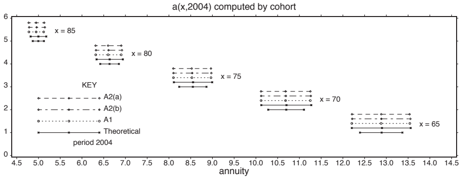
FIGURE 3B: (a) computations by cohort, period 2004, various ages (x).
