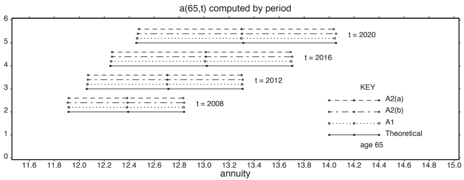
FIGURE 3B: (b) computations by period, age 65, various periods ( t > 2004 ).
