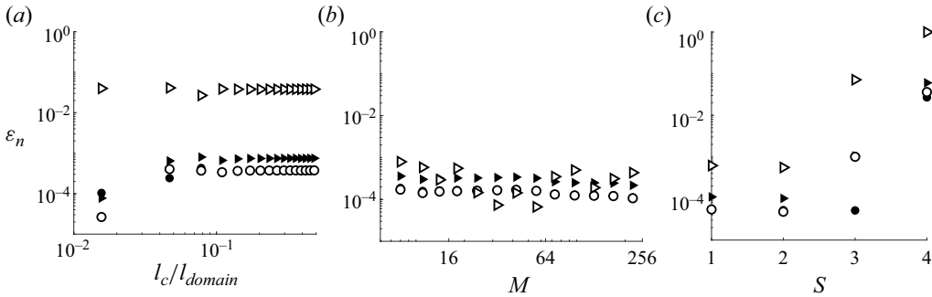
Figure 6. The relative error \varepsilon_n in the coefficients of the Navier–Stokes equation. (a) Dependence of \varepsilon_n on the spatial correlation length l_c . (b) Dependence of \varepsilon_n on the number of integration domains M . (c) Dependence of \varepsilon_n on the subsampling factor S . In all panels, the solid (hollow) triangles correspond to the pressure gradient \nabla p (viscous dissipation \nabla^2 \mathbf{u} ) and the solid (hollow) circles correspond to advection (\mathbf{u} \cdot \nabla)\mathbf{u} (time derivative \partial_t \mathbf{u} ).
