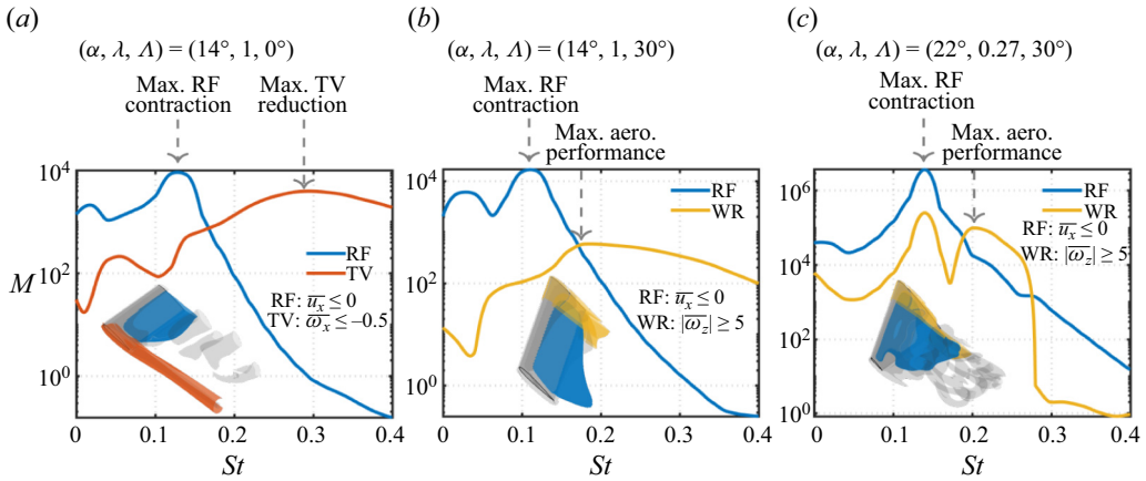
Figure 10. Assessment of control effects from response mode Reynolds stress metric M over St for (a) untapered unswept wing ( \lambda, \Lambda = 1, 0^\circ ) at \alpha = 14^\circ , (b) untapered swept wing ( \lambda, \Lambda = 1, 30^\circ ) at \alpha = 14^\circ and a (c) tapered swept wing ( \lambda, \Lambda = 0.27, 30^\circ ) at \alpha = 22^\circ . Grey arrows indicate frequencies in which controlled flows yielded maximum contraction of reversed-flow (RF) bubble, maximum tip vortex (TV) attenuation and maximum aerodynamic performance.
