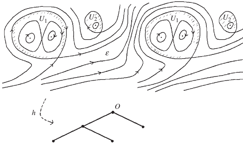
FIGURE 2. The stream lines of the flow and the corresponding graph.
