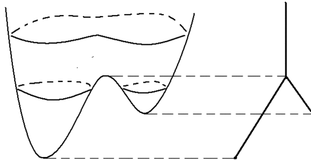
FIGURE 1. The graph of H and the corresponding graph \mathbb{G} .
