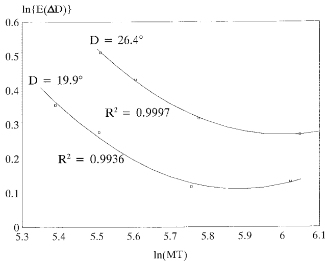
Figure R7. Best quadratic relationship between \ln\{E\{\Delta D\} and \ln MT as predicted by equation R3.7 using equation (68) to estimate E\{\Delta D\} . Data from Wright and Meyer (1983; Tables 2 and 4).
