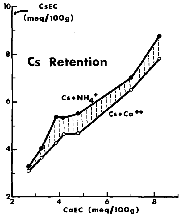
Figure 2. Cs retention of the kaolins ( \text{Cs}_{\text{NH}_4} - \text{Cs}_{\text{Ca}} ) as a function of their cation-exchange capacities.
