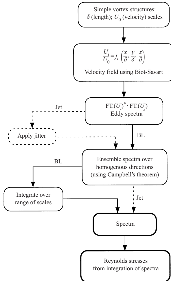
FIGURE 4. Procedure for calculating spectra from models.
