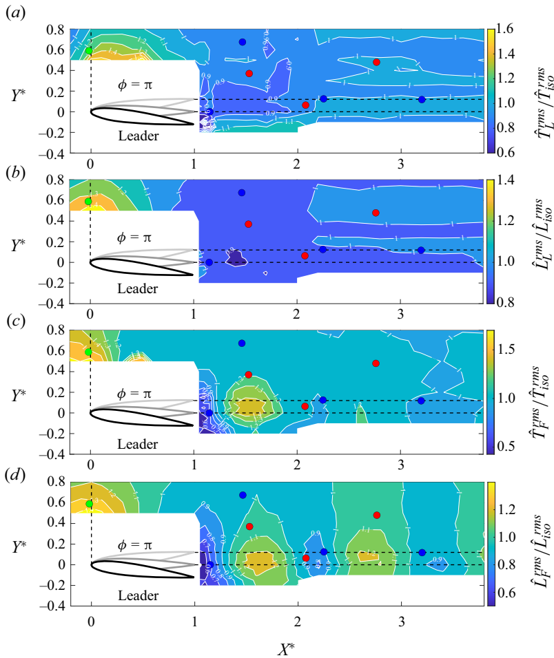
Figure 10. The r.m.s. of the fluctuating thrust and lift forces in the interaction plane normalised by the corresponding isolated foil metrics: for (a,b) the leader, and (c,d) the follower, where the fluctuating thrust and lift are defined as \hat{T} = T^{net} - \bar{T}^{net} and \hat{L} = L - \bar{L} , respectively. The subscripts L, F, iso denote leader, follower and isolated foil metrics, respectively. The green, blue and red circles represent the 2-D stable equilibria, the 1-D stable/1-D unstable saddle point equilibria, and the 2-D unstable equilibria, respectively, from figure 2.
