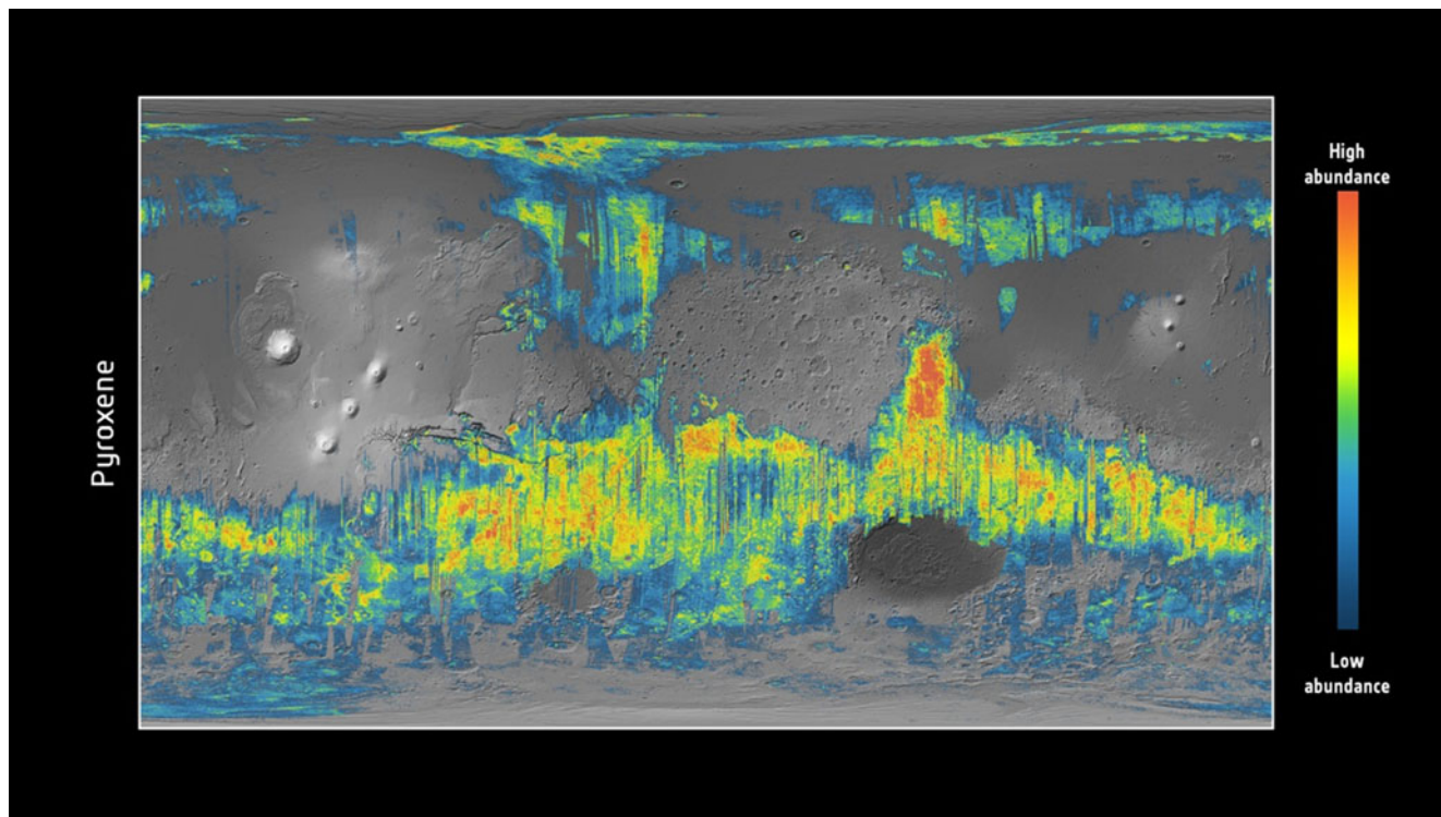
Fig. 4. Distribution of pyroxenes on the crust of Mars. Source: Bibring (2005).
