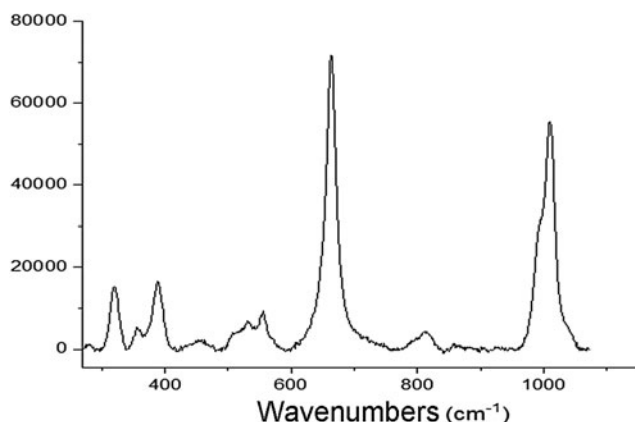
Fig. 2. Raman spectra of Zagami meteorite in this work.
