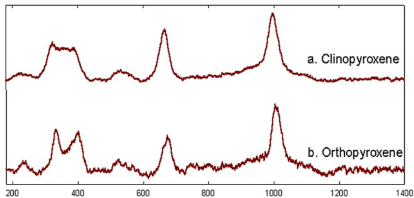
Fig. 3. Raman spectra of clinopyroxene and orthopyroxene minerals from the scientific literature. Source: Wang et al. (1999).
