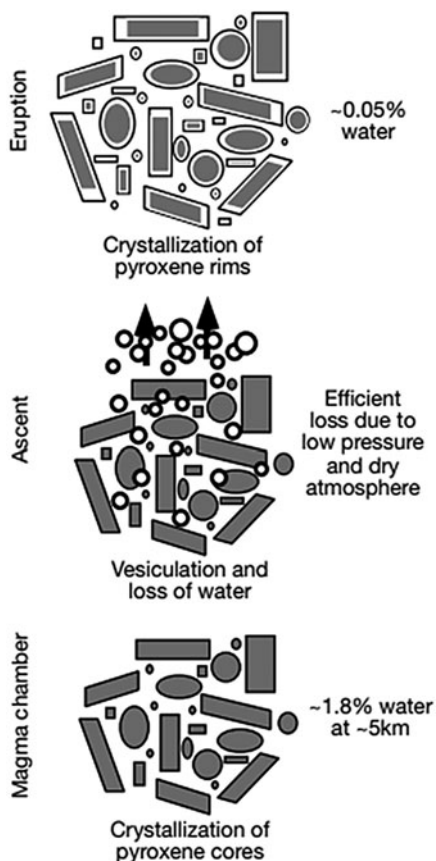
Fig. 5. Illustration of the process of crystallization of pyroxene during ascent and on eruption Fonte. Source: McSween et al. (2001).
