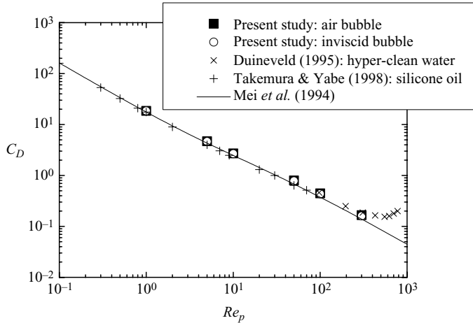
FIGURE 5. Drag coefficient, C_D , on an air bubble and an inviscid bubble in a uniform unsheared flow versus the particle Reynolds number, Re_p .
