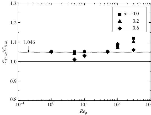
FIGURE 19. The ratio of the drag coefficient on a highly viscous bubble, C_{D, vb} , to that on an inviscid bubble, C_{D, ib} .
