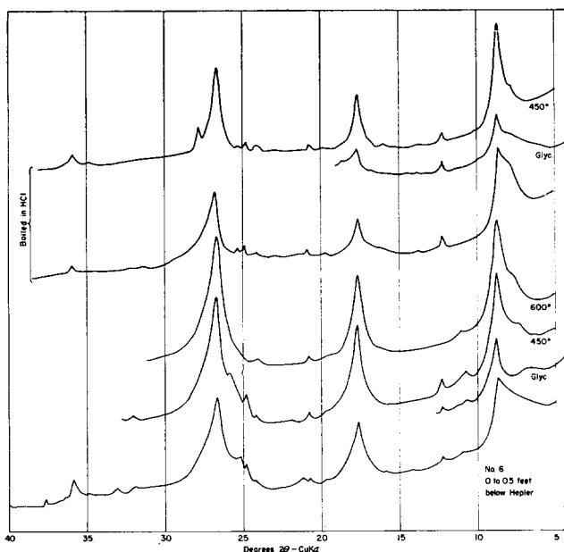
FIGURE 7.—X-ray diffractometer patterns of -2 micron fraction of shale immediately below Hepler (sample 6).
