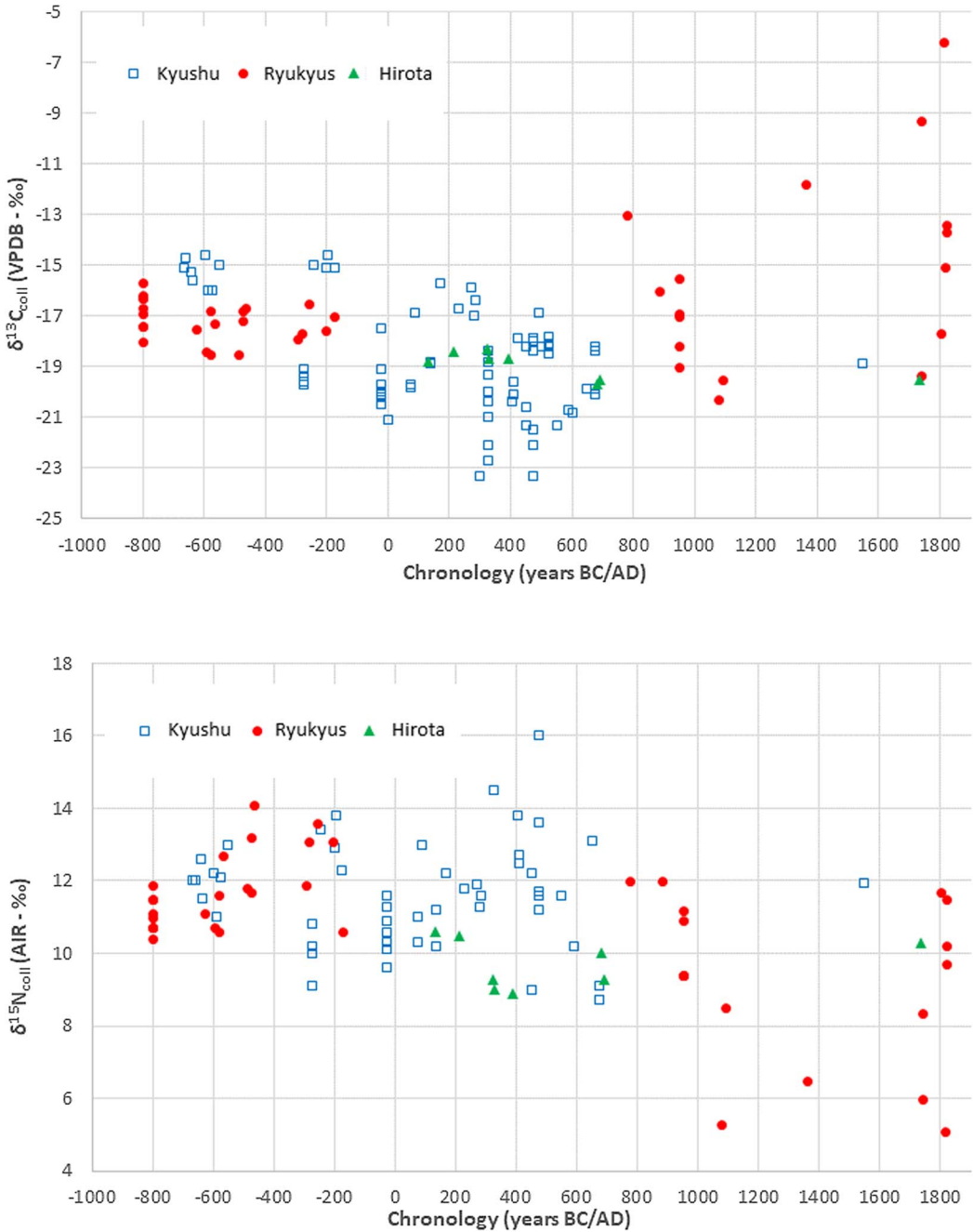
Figure 5. \delta^{13}C_{coll} (top) and \delta^{15}N_{coll} (bottom) values from human bone collagen from Kyushu and the Ryukyus, ca. 1000 BC to AD 1900. Data from Fernandes et al. (2021) with the date of the isotopic points set as the median of the chronological range given in the publication.
