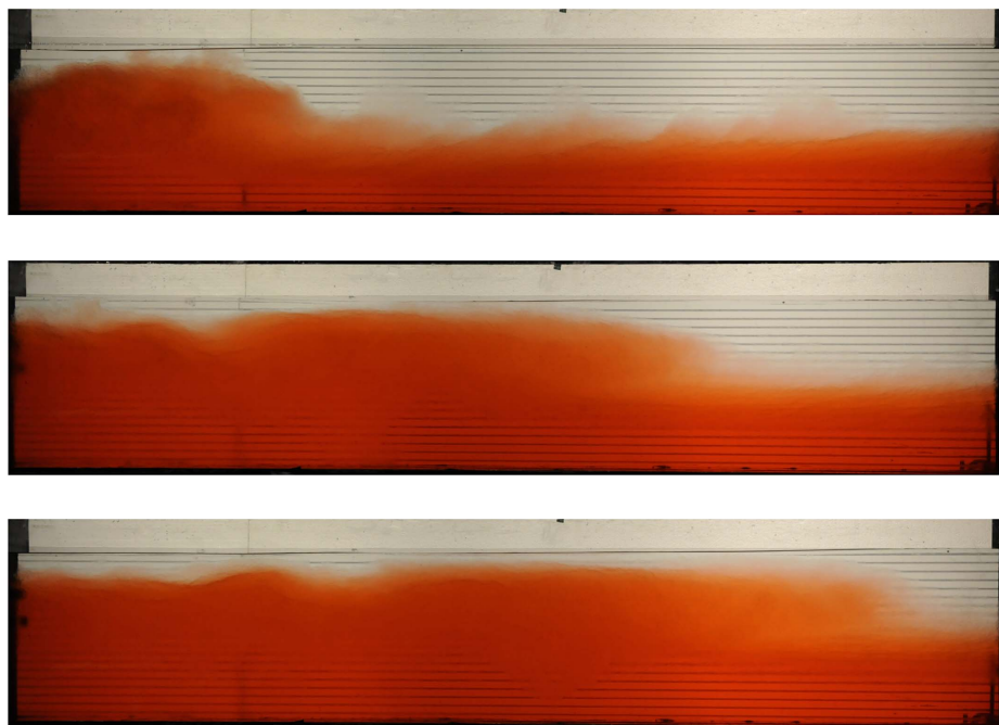
FIGURE 3. Visualization of the impact of the gravity current from Exp 6 – see table 1 – with the end wall of the channel and the subsequent internal bore that is generated. Note that the turbulence levels are significantly reduced from those for the current shown in figure 2.
