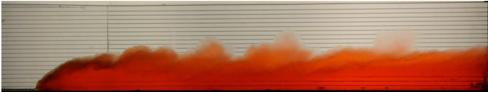
FIGURE 2. Visualization of the gravity current from Exp 6 – see table 1. The current is dyed with food colouring and viewed against a translucent lined sheet.
