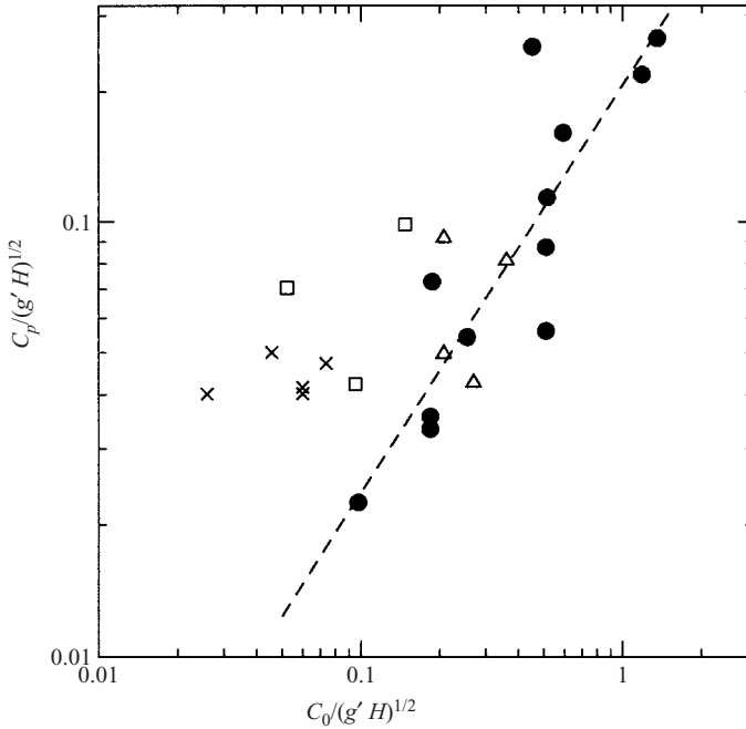
FIGURE 14. Phase speed of the unstable modes versus estimated upper-layer speed determined from PV conservation arguments. Symbols represent different ranges of \sigma , as in figure 12. The dashed line represents the best fit line through data with \sigma < 8 (solid circles).
