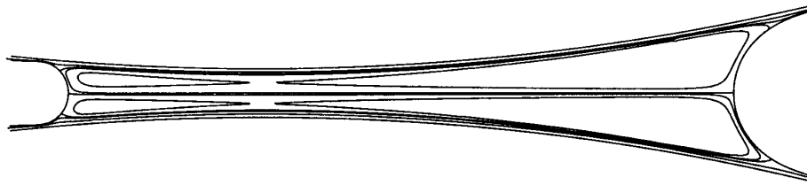
FIGURE 7. Streamlines for S = 1 , \zeta = 0.9 , \lambda = 0.1 , Ca = 0.01 , and R/B_0 = 100 : liquid is transferred from the lower to the upper roll via a transfer-jet snaking around both the two large eddies.
