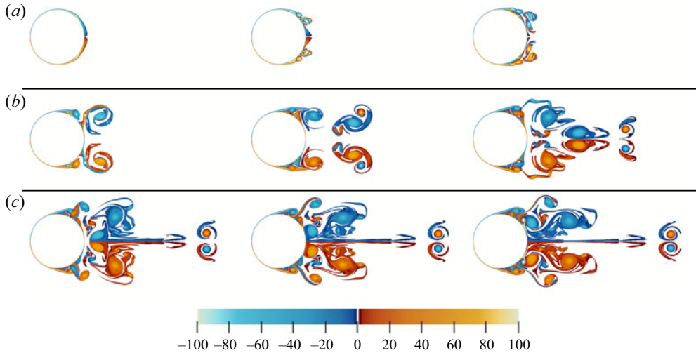
Figure 3. Vorticity field at Re = 25000 . Negative/positive vorticity is coloured with blue/orange. (a) t = 1.5T, 2.5T, 3.5T (vorticity eruption stage), (b) t = 5T, 7T, 9T (re-impingement of the wake dipole on the cylinder surface), (c) t = 10T, 10.4T, 10.8T (time when the dipole hits the cylinder and slides onto its surface).
