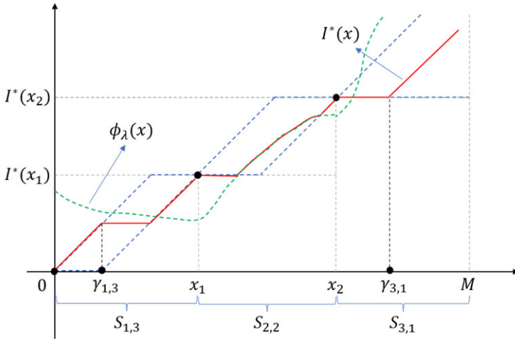
FIGURE 1: An illustration of an indemnity function I^* that solves problem (3.3), when m = 3, j_1 = 3, j_2 = 2 and j_3 = 1 .
