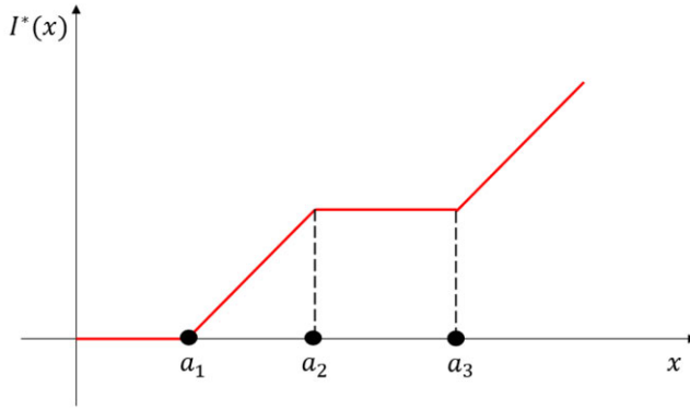
FIGURE 2: Illustrative I^* .
