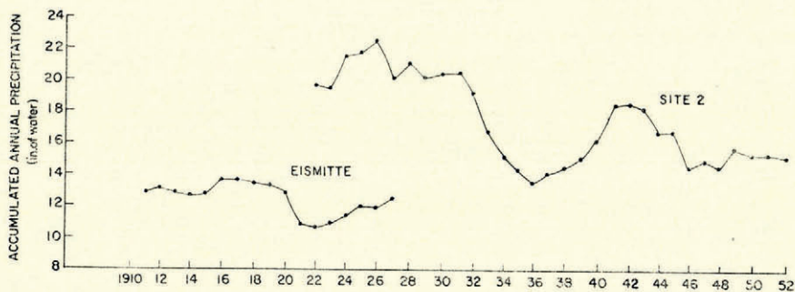
Fig. 4. Five-year moving means for accumulated annual precipitation at Site 2 and Eismitte. Points are plotted on middle year of each 5-year period
