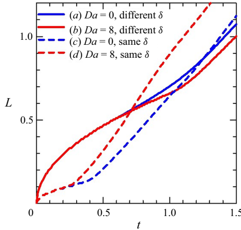
Figure 13. Mixing length of non-reactive ( Da = 0 ) and reactive VF ( Da = 8 ) patterns for Pe = 1000 with different ( \delta_A = \delta_E = 10, \delta_b = 1 , solid lines) or same diffusivity ( \delta_A = \delta_E = 1, \delta_b = 1 , dashed lines). The curves show the average of five data with different initial perturbations.
