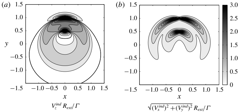
FIGURE 17. Induced velocity contours in a cross-section ( z=0 plane) for h^*=1 , R^*=0.5 , \alpha=1.5 , \varepsilon=0.03 , N=1 and \kappa=1 . In (a) colours are for |V_z^{ind}| with the same colour map as in (b).
