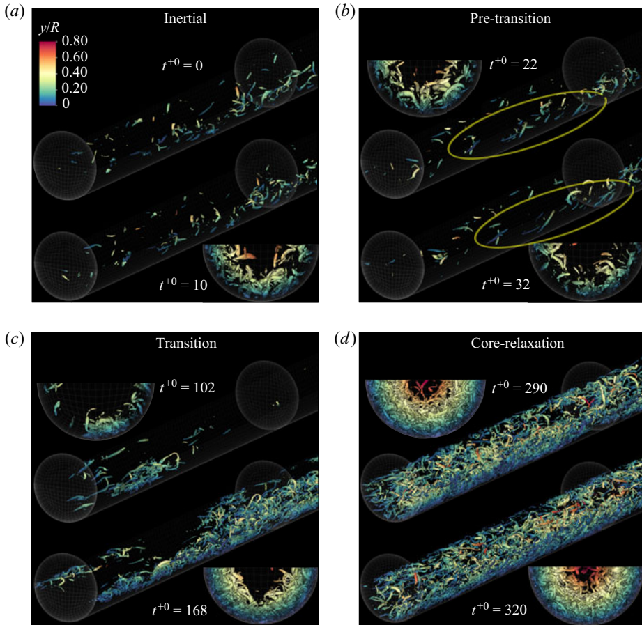
Figure 3. Temporal evolution of the vortical structures for case TP2 based on the \lambda_2 criterion. The isosurfaces are coloured by the wall-normal distance y/R . (a) inertial stage, (b) pre-transition, (c) transition and (d) core relaxation. The yellow ellipses in (b), during the pre-transition stage, highlight a region where several quasi-streamwise vortices are stretched between two consecutive snapshots. Note that in all the snapshots, only the lower half of the pipe is displayed for clarity.
