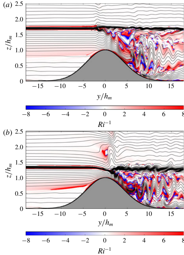
FIGURE 8. Instantaneous snapshots of the inverse Richardson number overlain with isopycnal contours. (a) Flat interface ( z_0 = 1.73h_m ) and (b) plunging interface ( z_0 = 1.33h_m ).
