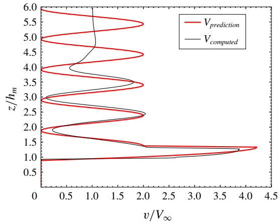
FIGURE 7. Same as figure 5 but for z_0 = 1.33h_m . The prediction for the peak speed is obtained from (3.8), while the wave aloft is assumed to have a vertical wavelength 2\pi V_\infty/N_0 and perturbation speed amplitude of V_\infty (see § 6.1). The phase of the wave is chosen to match the computed solution.
