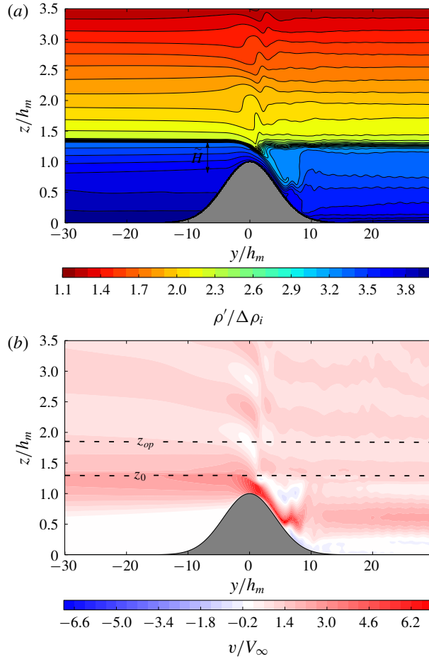
FIGURE 6. Same as figure 4 but for z_0 = 1.33h_m .
