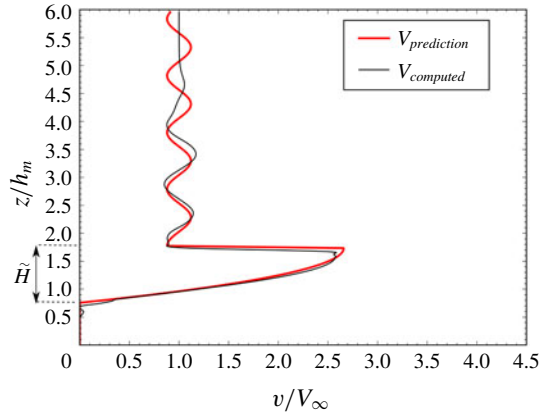
FIGURE 5. Vertical profile of the steady streamwise velocity at the blocking point y = -y_b for Fr = 0.16 flow over an infinite ridge with a sharp density step located at z_0 = 1.73h_m . The prediction in red is based on the values of \tilde{H} and v_m from (3.5) and (3.6), respectively. The wave aloft is predicted to have a vertical wavelength 2\pi V_\infty/N_0 and perturbation speed amplitude V_\infty N_0/N_{\delta_i} = 0.12V_\infty (see § 6.1), with the phase chosen to match the computed solution.
