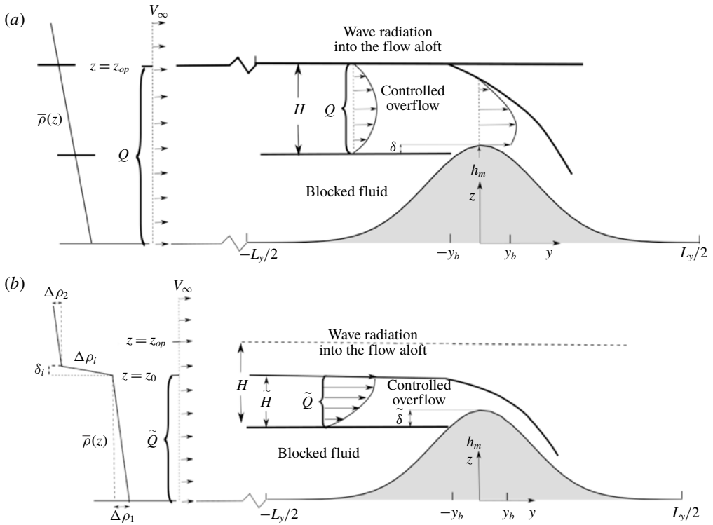
FIGURE 1. (a) Schematic of low Fr controlled asymmetric overflow over an infinite ridge for the case of uniform upstream stratification and flow speed. The upstream fluid below a depth \delta from the crest is blocked. The streamwise coordinate of the blocking location is y = -y_b , and Q denotes the volume transport within the overflow, which matches the far upstream transport as shown. The streamwise computational boundaries are y = -L_y/2 and y = L_y/2 . The optimally controlled overflow has a parabolic velocity profile, with the height of the bifurcating isopycnal being z = z_{op} . Panel (b) is as in figure 1(a) but for the case when a density step is present in an otherwise uniformly stratified fluid with Fr = V_\infty/N_0 h_m \ll 1 . The density step \Delta\rho_i is large and the interface is thin relative to H ( \delta_i/H \ll 1 ), so that N_{\delta_i}/N_0 \gg 1 , where N_{\delta_i} and N_0 denote the stratification within and away from the interface, respectively. The flow arrows indicate that the far upstream inflow speed is a constant V_\infty up to an arbitrary height z > z_{op} . For z = z_0 < z_{op} , the upstream thickness of the overflow is \tilde{H} < H and the velocity profile deviates from the optimal parabolic shape as indicated. Note that the downward arrows associated with H and \tilde{H} point to different z locations. This is in anticipation of the result (see also, §3) that the blocking scale \tilde{\delta} when the isopycnal bifurcates at the vertical level of the density step is different from the blocking scale \delta when no density step is present.
