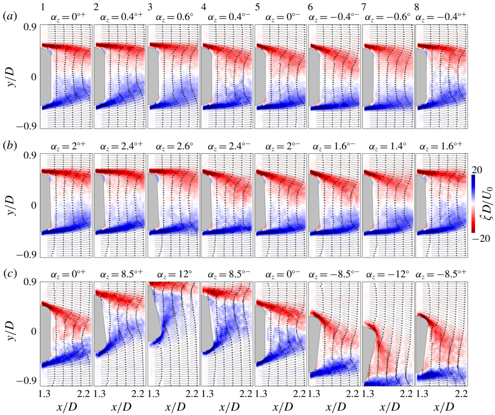
FIGURE 19. (Colour online) Colour raster plots of the phase-averaged azimuthal vorticity concentrations \hat{\xi} with overlaid velocity vectors in the near wake (at eight equal time increments 0.125\tau_z apart, 0 < t/\tau_{z-act} < 0.875 ) in the presence of closed-loop control corresponding to figure 17(a–c): attitude stabilization about \alpha_z = 0^\circ ( \tau_{z-act} = \tau_{z,0} = 0.3\tau_z , (a), and 2^\circ ( \tau_{z-act} = \tau_{z,2} = 0.4\tau_z , b), and oscillation amplification ( \tau_{z-act} = \tau_{z-amplify} = 1.25\tau_z , (c)).
