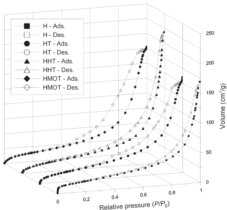
Figure 12. N_2 adsorption/desorption isotherms at 77 K for the 'Dunino' halloysite (<math><2 \mu\text{m}</math>) (H) and its derivatives HT, HHT, and HMOT.
