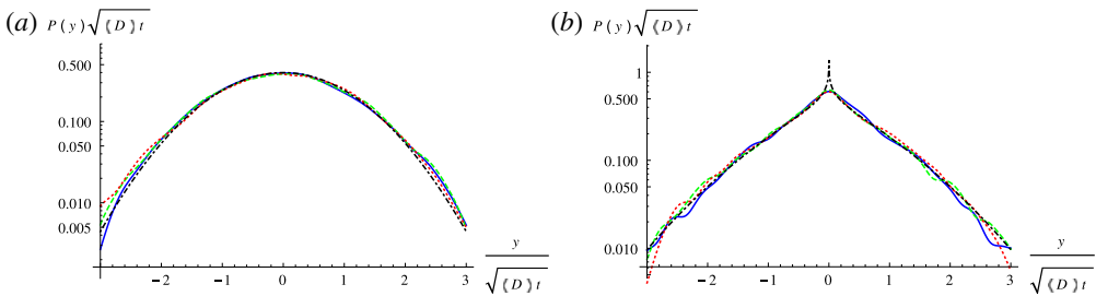
FIGURE 8. Rescaled PDF as a function of the similarity variable x = y/\sqrt{\langle D \rangle t} for 3 different times t = 500 (solid blue), t = 1000 (dashed green) and t = 5000 (dotted red) for the values of \rho_{th} = 0.1 (a) and \rho_{th} = 1 (b). They all collapse to a single function that depends on \rho_{th} . Theoretical curves are black dashed.
