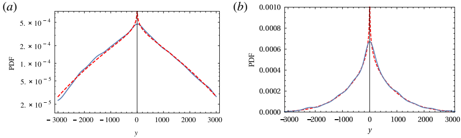
FIGURE 5. PDF from (3.6) (dashed red) for \rho_{th} = 1 and A = 20 in log-linear (a) and linear (b) scales fitting the numerically obtained PDF for the same parameters (blue).
