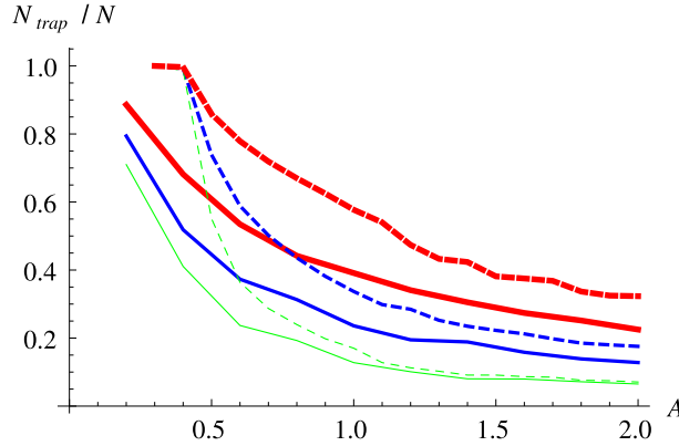
FIGURE 3. Trapped particle fraction (i.e. particles not reaching a surface at r = 10 after 100 iterations) from a thermal distribution of Larmor radii for three values of the thermal radius: \rho_{th} = 0.7 (green), 1 (blue) and 1.5 (red). Dashed lines are for the initial population at elliptical point (0,0) , continuous lines for hyperbolic point (\pi/2, \pi/2) .
