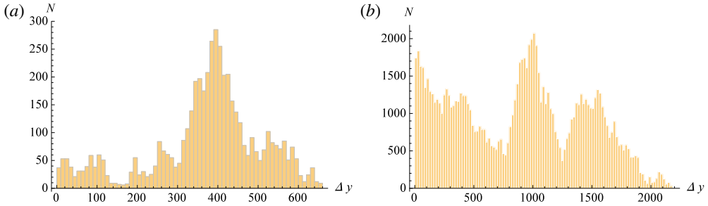
FIGURE 11. Histograms for the step length sizes |y_{n+1} - y_n| in the chaotic regime with flow. There is a large contribution of very long jumps whose mean size strongly increases with time: (a) is for N = 5000 iterations of the map while (b) is for N = 10^5 .
