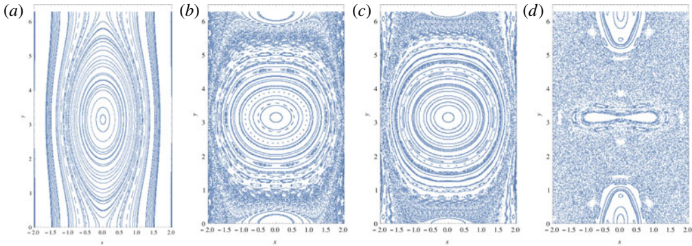
FIGURE 10. Phase space trajectories for the mapping with flow when C=0.5 . (a) \rho = 0 and A = 0.02 ; (b) \rho = 0 and A = 0.1 ; (c) \rho = 0.5 and A = 0.1 ; (d) \rho = 0.5 and A = 0.3 . The streaming regular motion for small wave amplitude and \rho becomes chaotic as A grows.
