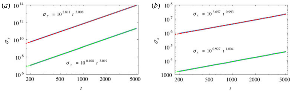
FIGURE 12. (a) Variance of the y displacements for thermal particles with \rho_{th} = 1 as function of time in log–log scale, showing the cubic scaling for A = 1 (lower curve) and A = 20 (upper curve). (b) Variance for x for the same cases of (a). The regression fit is shown with dashed lines together with the corresponding equation.
