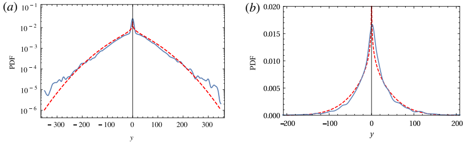
FIGURE 4. PDF of displacements in y of an ensemble of particles with a Maxwellian distribution of Larmor radii in (3.2) (continuous blue line) with A = 1 , \rho_{th} = 1 , in log-linear scale (a) and in linear scale (b). The dashed red line is the fit from (3.6). The long tails indicate an exponential-like decay as opposed to the Gaussian decay characteristic of ensembles with zero Larmor radii. Also the relatively high value of the kurtosis, K = 6.56 , indicates strong departures with respect to the K = 3 Gaussian case without FLR effects.
