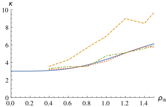
FIGURE 9. Dependence \kappa(\rho_{th}) of the kurtosis on the thermal radius: the theoretical dependence from (3.12) (solid blue) and the numerical dependences for A = 1 (dashed orange), A = 5 (dot-dashed green) and A = 20 (dotted red).
