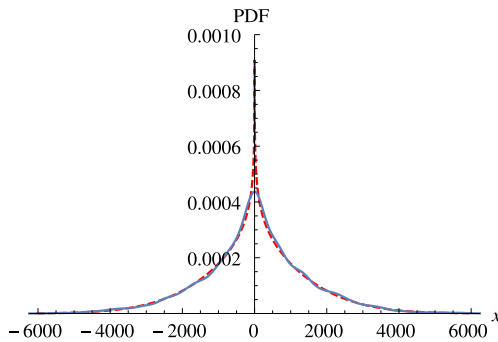
FIGURE 15. PDF for the x -direction for \rho_{th} = 1 , A = 20 and C = 0.7 obtained from (3.6) using the value of D from (3.5) (dashed red) fitting the numerically obtained PDF for the same parameters (solid blue).
