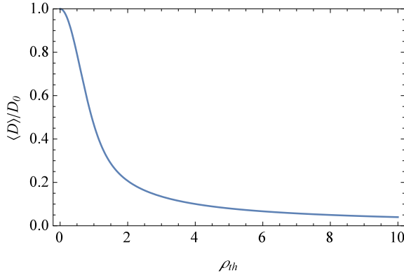
FIGURE 7. Effective diffusion coefficient for the transport associated with the PDF in (3.6).
