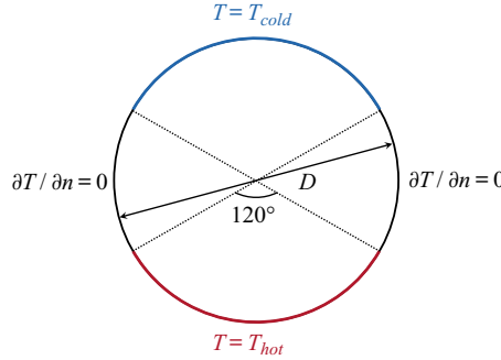
FIGURE 1. Schematic illustration of the 2-D circular convection cell.
