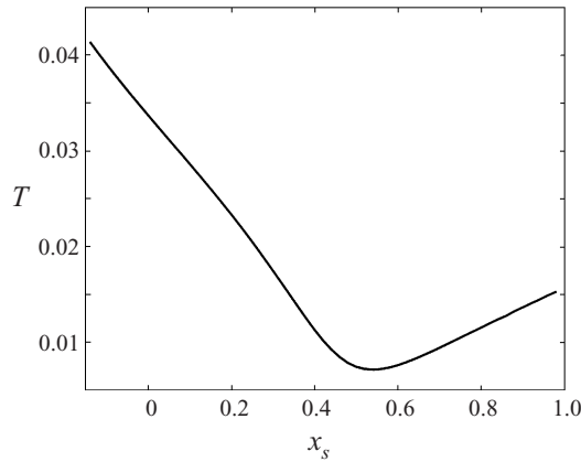
FIGURE 2. The variation of T as a function of x_s when \Gamma_c = 30 and x_c = -0.15 .
