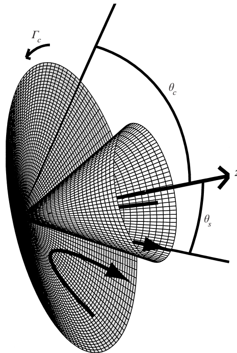
FIGURE 1. The geometry of the two-cell flow case. The symmetry axis is in the z -direction, \theta_c is the angle of the bounding streamsurface and \Gamma_c is the circulation thereon. \theta_s is the angle of the streamsurface, which separates the two cones. The thick arrows indicate the direction of the radial velocity component.
