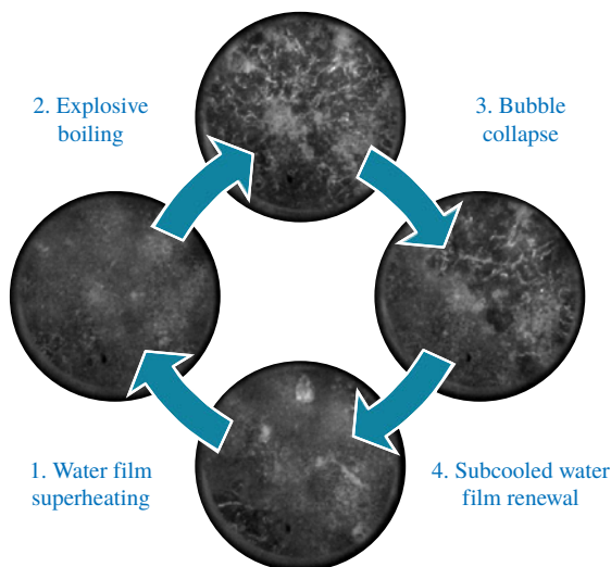
FIGURE 11. Liquid contact hypothesis: cyclic explosive boiling and condensation.
