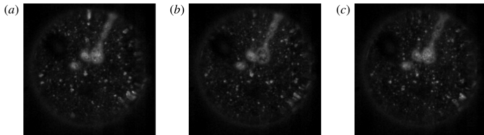
FIGURE 5. Flashing frequency on a smooth plate (see brightness changes in central patch); initial plate temperature of 650^{\circ}\text{C} and water jet at 25^{\circ}\text{C} . The circle corresponds to the 9 mm diameter stagnation zone. Time after impingement: (a) 23.284 ms; (b) 23.420 ms; (c) 23.469 ms.
