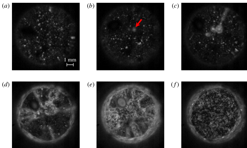
FIGURE 4. Rewetting during smooth plate quenching; initial plate temperature of 650^{\circ}\text{C} and water jet at 25^{\circ}\text{C} . The circle corresponds to the 9 mm diameter stagnation zone. Time after impingement: (a) 7.852 ms; (b) 19.555 ms; (c) 23.457 ms; (d) 31.617 ms; (e) 39.420 ms; (f) 63.185 ms.
