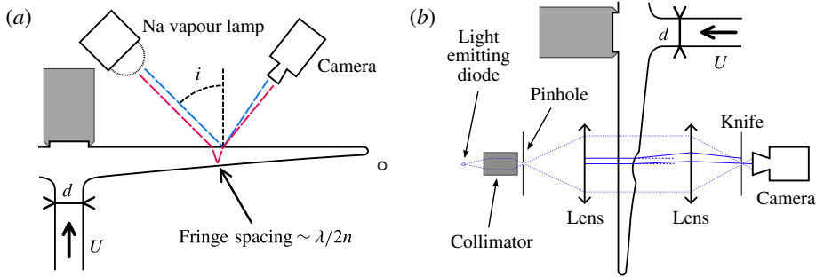
FIGURE 4. (Colour online) Visualisation techniques. (a) Interferometry: a sodium vapour lamp imprints stripes on the sheet. Two consecutive fringes are separated by a constant thickness jump \Delta h = \lambda/2n \cos i_r , with i_r the refracted angle inside the sheet. (b) Schlieren: modulations of the thickness of the sheet, located in the plane of observation, deviate parallel light as would optical lenses.
