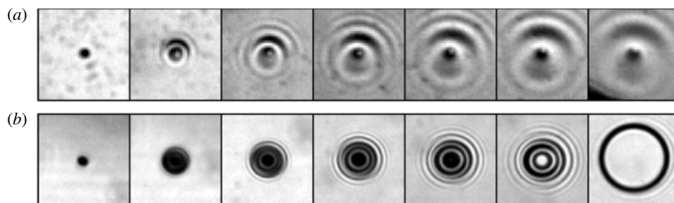
FIGURE 7. (a) Water droplet falling on a moving water film ( U = 3.8 \text{ m s}^{-1} ) with thickness h = 14 \text{ } \mu\text{m} , and generating capillary waves. Pictures are 3.6 \text{ mm} wide, recorded every 700 \text{ } \mu\text{s} . (b) Ethanol droplet falling on a moving water film ( U = 3.9 \text{ m s}^{-1} ) with thickness h = 13 \text{ } \mu\text{m} , and piercing it. Pictures are 5.8 \text{ mm} wide, recorded every 500 \text{ } \mu\text{s} .
