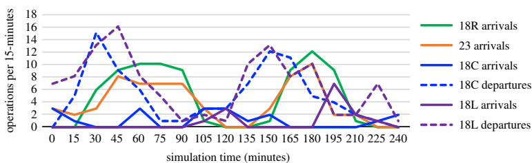
Figure 3. Runway demand.
