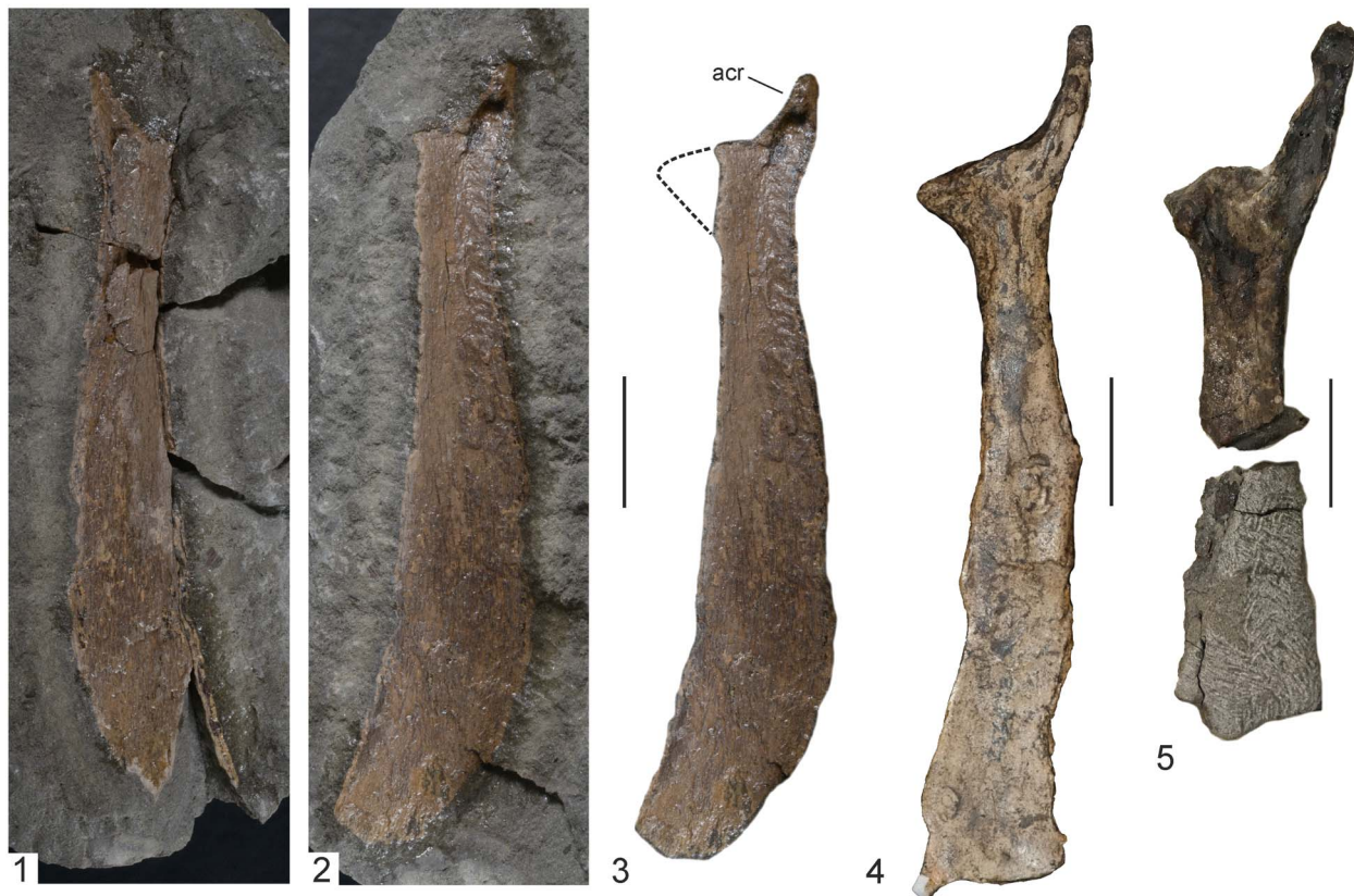
Figure 1. (1–3) cf. Tonsala hildegardae (SMF Av 662) left scapula compared with (4) a cast of the right scapula of the holotype (LACM 123791) and (5) the left scapula of gen. indet. sp. indet. A (UWBM 86871); in (3), the surrounding matrix was digitally removed. acr = acromion. Scale bars = 20 mm.
