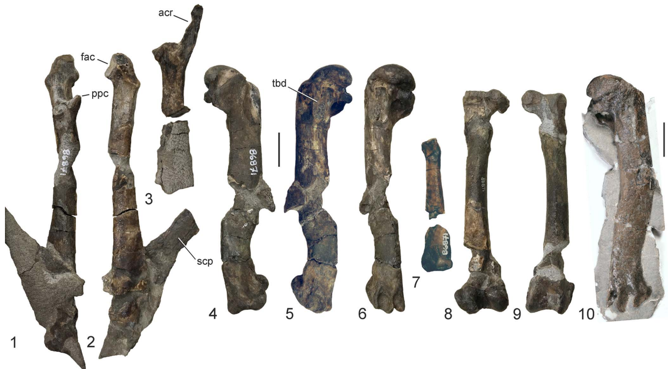
Figure 3. (1–9) Major bones of the plotopterid specimen UWBM 86871 from the Makah Formation (gen. indet. sp. indet. A), which was previously assigned to, and in part used to diagnose (incorrectly), Tonsala buchani by Dyke et al. (2011). (1, 2) Left coracoid: (1) dorsal view; (2) ventral view. (3) Cranial portion of the left scapula in lateral view. (4–6) Left humerus: (4) cranial view; (5) caudal view; (6) caudoventral view. (7) Proximal and distal portions of left ulna. (8, 9) Left femur: (8) caudal view; (9) cranial view. (10) Right humerus, which is here assigned to the same indeterminate species (SMF Av 650). acr = acromion; fac = facies articularis clavicularis; ppc = processus procoracoideus; scp = portion of scapular blade; tbd = tuberculum dorsale. Scale bars = 20 mm.
