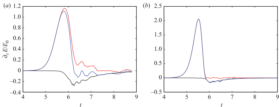
FIGURE 3. Energy balance for the fluctuations in spin-down ( Re_{eff} = 2200 ): (a) BOUS ( Ro_r = 0.5 ); (b) QG. Blue is the total rate of change of the fluctuations, red is the energy conversion from mean to fluctuations, and black is the dissipation of fluctuation energy.
