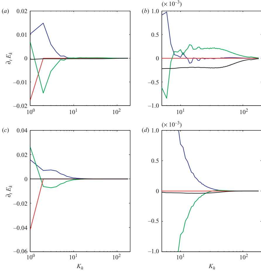
FIGURE 14. Kinetic energy balance in spectral space ( Re_{eff} = 2200 ): BOUS ( Ro_r = 0.5 , a,b ) and QG ( c,d ). Terms are conversion of potential energy (blue), advective flux divergence (green), restoring damping of wavenumber 1 (red) and dissipation (black). Panels ( b,d ) have an expanded ordinate for the higher wavenumbers.
