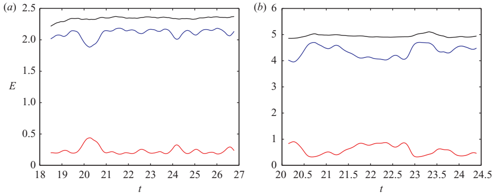
FIGURE 5. Time series of total kinetic plus available potential energy (black) and its mean (red) and fluctuation (blue) components for Re_{eff} = 2200 with restoring forcing during equilibrium: (a) BOUS ( Ro_r = 0.5 ); (b) QG.
