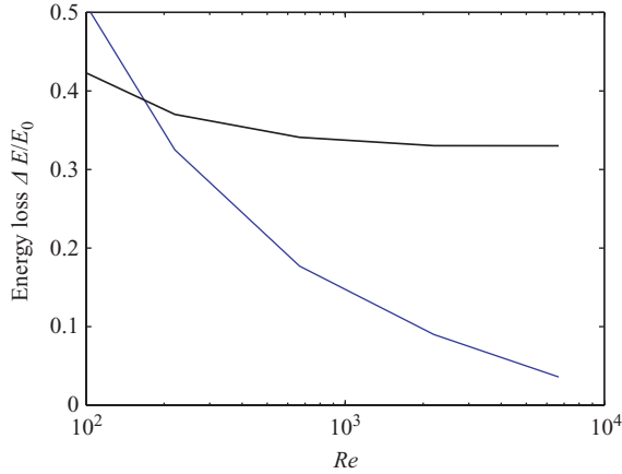
FIGURE 4. Total energy loss during spin-down for different values of Re_{eff} : BOUS ( Ro_r = 0.5 , black) and QG (blue).
