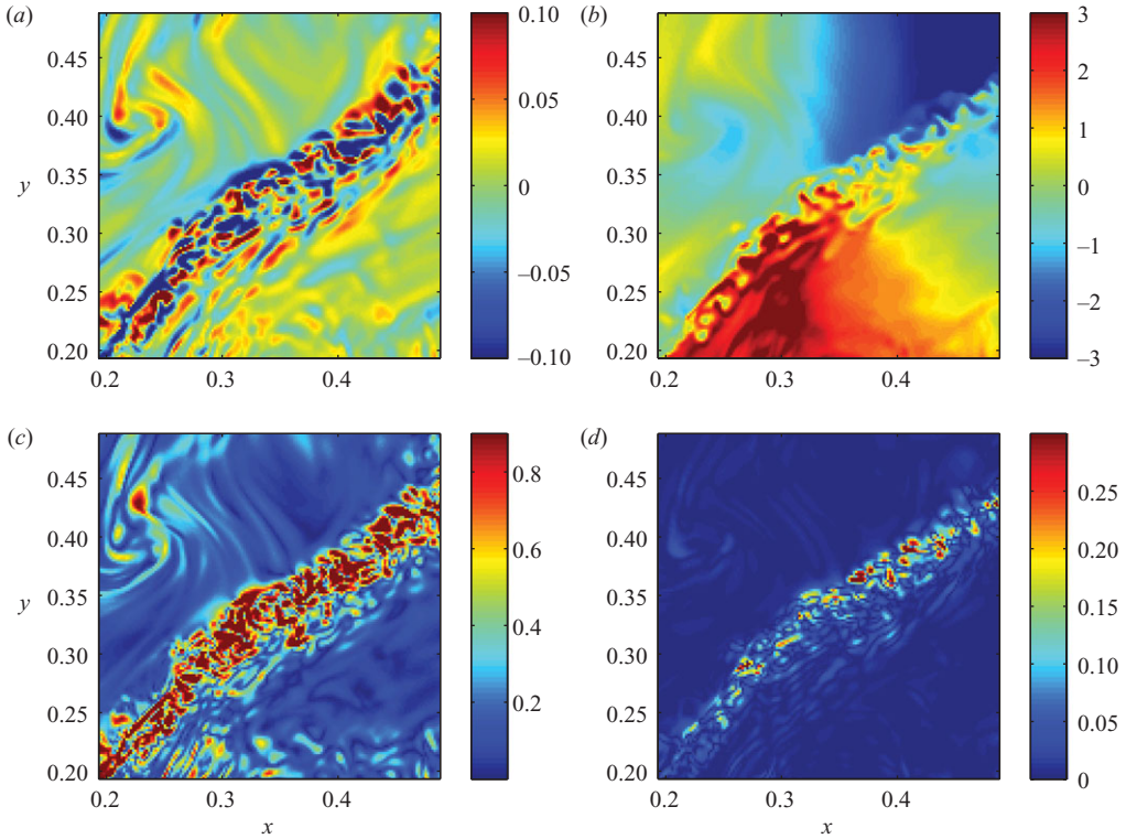
FIGURE 17. A local region with submesoscale frontal instability in BOUS ( z = 0.96 , Ro_r = 0.5 , Re_{eff} = 6600 ). The format is the same as in figure 16.
