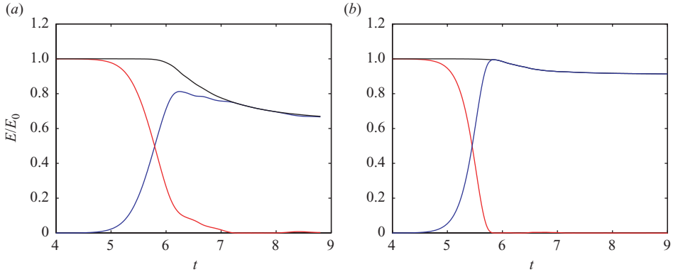
FIGURE 1. Evolution of total energy (kinetic plus available potential) in spin-down ( Re_{eff} = 2200 ): (a) BOUS ( Ro_r = Fr = 0.5 ); (b) QG. Blue is the fluctuation energy, red is the basic-state energy, and black is the total energy. Towards the end of the simulation, all the kinetic and available potential energy from the basic state is depleted, and the fluctuations have evolved towards a flow structure that fills the domain and is only weakly dissipative.
