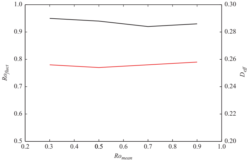
FIGURE 12. Fluctuation Rossby number Ro_{fluct} (measured by the r.m.s. value of the non-dimensional fluctuation vertical vorticity multiplied by Ro ; left ordinate and black curve) and dissipation efficiency (right ordinate and red curve) as functions of mean Rossby number Ro_{mean} = Ro_r . ( Re_{eff} = 2200 .)
