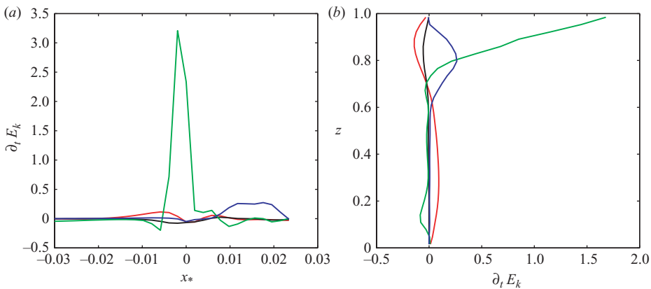
FIGURE 20. Energetics of the frontal instability in figure 19. (a) Cross-frontal profiles for depth-averaged kinetic energy production terms and (b) vertical profiles averaged over the cross-frontal direction. The production terms are \overline{(u'_* v'_*) v_{*x}} (green), \overline{(w v'_*) v_{*z}} (blue), \overline{(W b')} (black) and \overline{w \mathcal{B}} (red).
