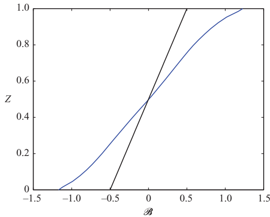
FIGURE 8. Mean buoyancy profile \mathcal{B} in BOUS ( Ro_r = 0.5 , Re_{eff} = 2200 ): black is the basic-state stratification (equal to the permanent QG stratification), and blue is the averaged stratification after equilibration.
