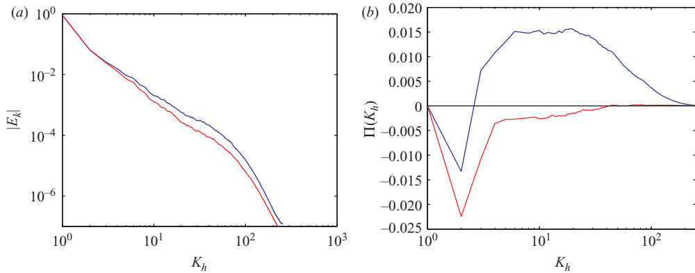
FIGURE 18. (a) Three-dimensional kinetic energy spectrum of \mathbf{u} for the BOUS solution (blue) and its horizontally non-divergent counterpart \mathbf{u}_{nd} (red). (b) Spectral flux of kinetic energy for BOUS velocity (blue) and a projected horizontal velocity with \nabla_h \cdot \mathbf{u}_h = 0 (red). ( Ro_r = 0.5 ; Re_{eff} = 6600 .)
