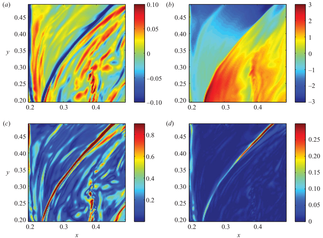
FIGURE 16. A local region with \sim stable submesoscale frontogenesis in BOUS ( z=0.96 , Ro_r=0.5 , Re_{eff}=6600 ): (a) vertical velocity, (b) buoyancy, (c) error in gradient wind balance \varepsilon_{gw} and (d) error in hydrostatic balance \varepsilon_{hydro} .
