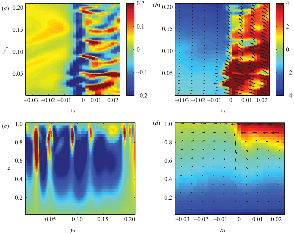
FIGURE 19. A local view of an unstable frontal region. (a) Near-surface, horizontal slice for vertical velocity. (b) The same for buoyancy with overlaid horizontal velocity vectors. (c) Vertical, along-frontal section for vertical velocity at x_* = 0 . (d) Vertical, cross-frontal section of along-front averaged buoyancy and velocity vectors. The local volume-averaged velocity has been subtracted from \mathbf{v} to expose the frontal circulation.
