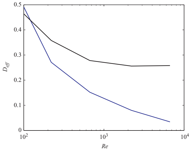
FIGURE 11. Dissipation efficiency as a function of Re_{eff} : BOUS ( Ro_r = 0.5 , black) and QG (blue).
