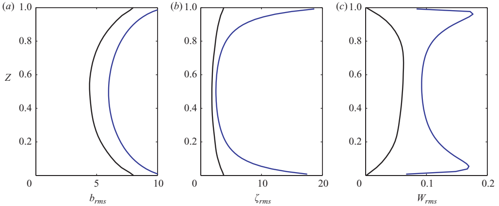
FIGURE 9. RMS profiles of b , \zeta^z and w in equilibrium ( Re_{eff} = 2200 ): BOUS ( Ro_r = 0.5 , black) and QG (blue).
