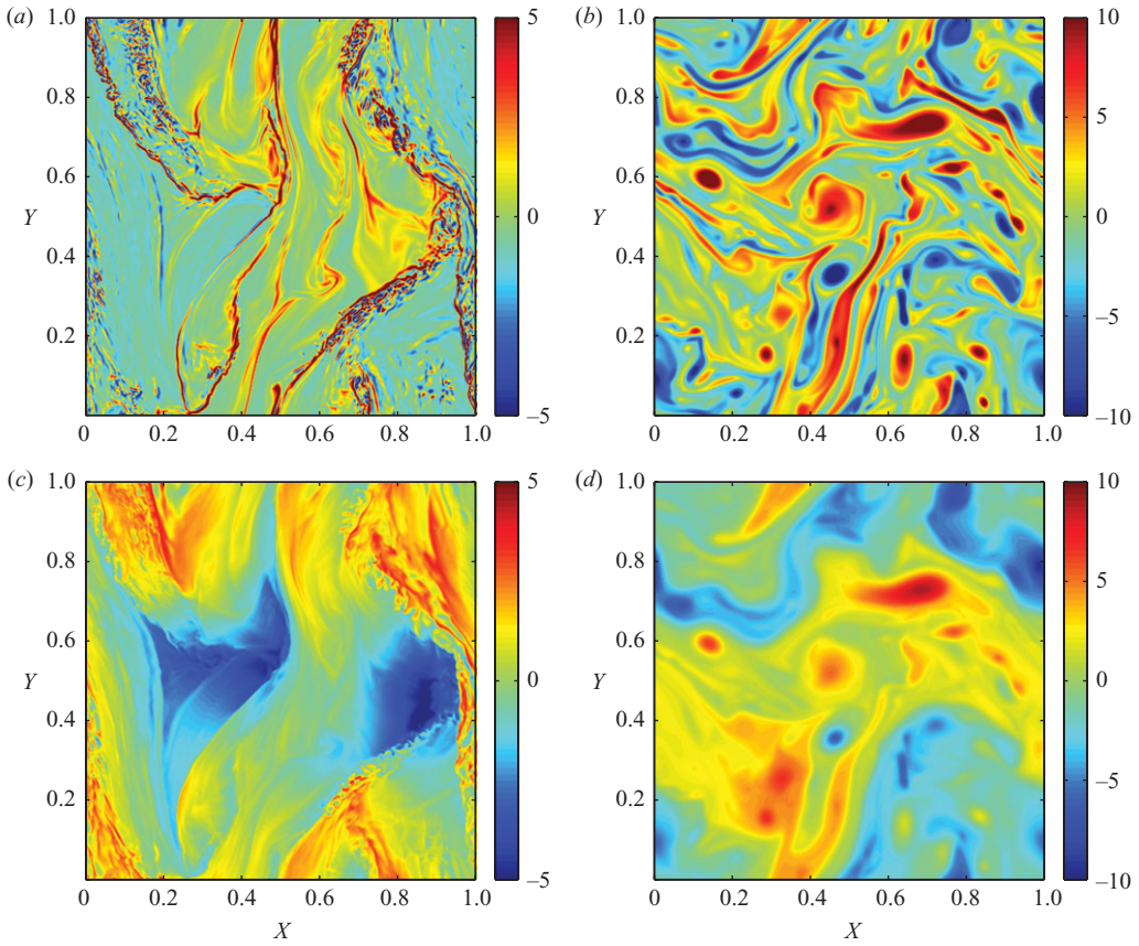
FIGURE 7. Snapshots in equilibrium ( t = 100 ) at z = 0.96 for Re_{eff} = 2200 : BOUS ( Ro_r = 0.5 ) \zeta^z (a) and b (c); the same for QG in (b,d). Note the fine-structure present in BOUS.
