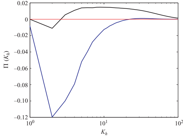
FIGURE 15. Spectral flux of kinetic energy ( Re_{eff} = 6600 ): BOUS ( Ro_r = 0.5 , black) and QG (blue). Note the forward cascade for BOUS and inverse cascade for QG.
