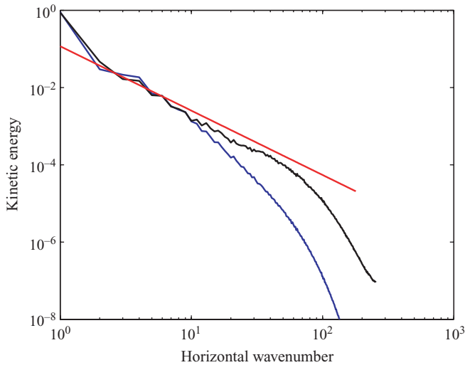
FIGURE 13. Time- and depth-averaged horizontal kinetic energy spectra ( Re_{eff} = 6600 ): BOUS ( Ro_r = 0.5 , black) and QG (blue). Spectra are normalized by the mean of kinetic energy \mathcal{E}_k . A red line \propto k^{-5/3} is plotted for comparison.
