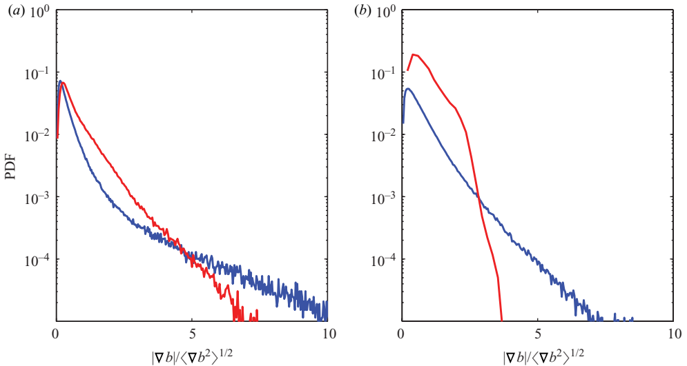
FIGURE 10. PDF of |\nabla b| in the interior (red) and near the boundary (blue) ( Re_{eff} = 2200 ): BOUS ( Ro_r = 0.5 , a ) and QG ( b ). The PDF is normalized to have unit integral and unit variance. The interior is defined as 0.375 < z < 0.625 , and the near-boundary as z < 0.125 or z > 0.875 . Average r.m.s. values are \nabla b_{rms} = 0.51 (BOUS interior), \nabla b_{rms} = 1.11 (BOUS near-boundary), \nabla b_{rms} = 0.05 (QG interior) and \nabla b_{rms} = 1.07 (QG near-boundary).
