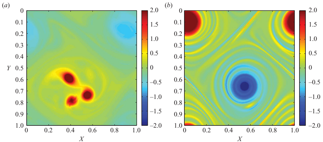
FIGURE 2. Vertical vorticity \zeta^z(x, y) at t=9 and z=0.5 in spin-down ( Re_{eff} = 2200 ): (a) BOUS ( Ro_r = 0.5 ), where the fluctuations have evolved to a set of co-rotating cyclonic eddies; (b) QG, where the fluctuations have evolved to a dipole vortex structure.
