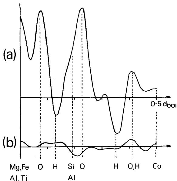
Figure 1. (a) Variation of neutron scattering density along the perpendicular to the vermiculite sheets. (b) Difference ( F_{\text{obs}} - F_{\text{calc}} ) neutron scattering density. Scale = same as in (a).
