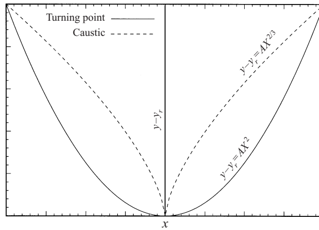
FIGURE 14. Approximated ray paths near the reflection levels. The tangents to the rays are vertical at turning points while they are horizontal at the caustics.
