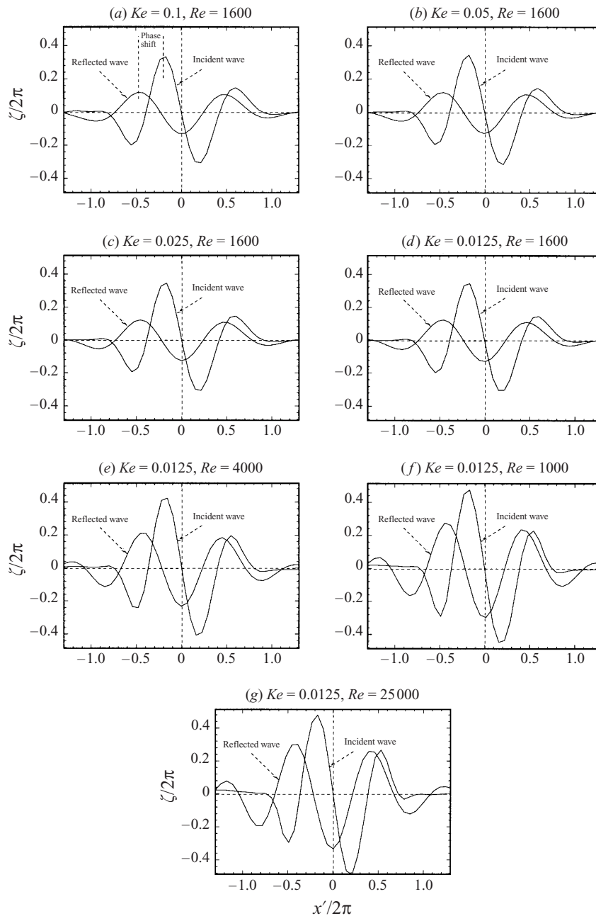
FIGURE 3. The waveforms of the internal wave before and after the reflection. The origin of the x' -axis corresponds to the position at which the maximum amplitude of the incident wave occurs and the group velocity is pointing in the direction of increasing y' . At the centre of the wave beam, a phase shift of \pi/2 occurs when internal waves reflect.
