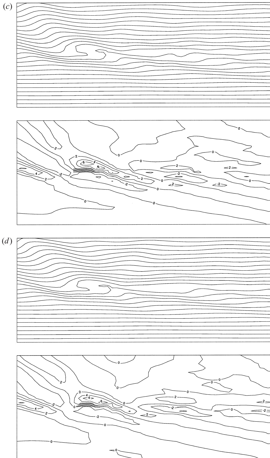
FIGURE 23. Density and vorticity contour plots for Ke = 0.3 , shading indicates the regions of Ri_t < 1/4 . The strong shear regions correspond to Ri_t < 1/4 . (a) T = 7 , (b) T = 8 , (c) T = 9 , (d) T = 10 .
