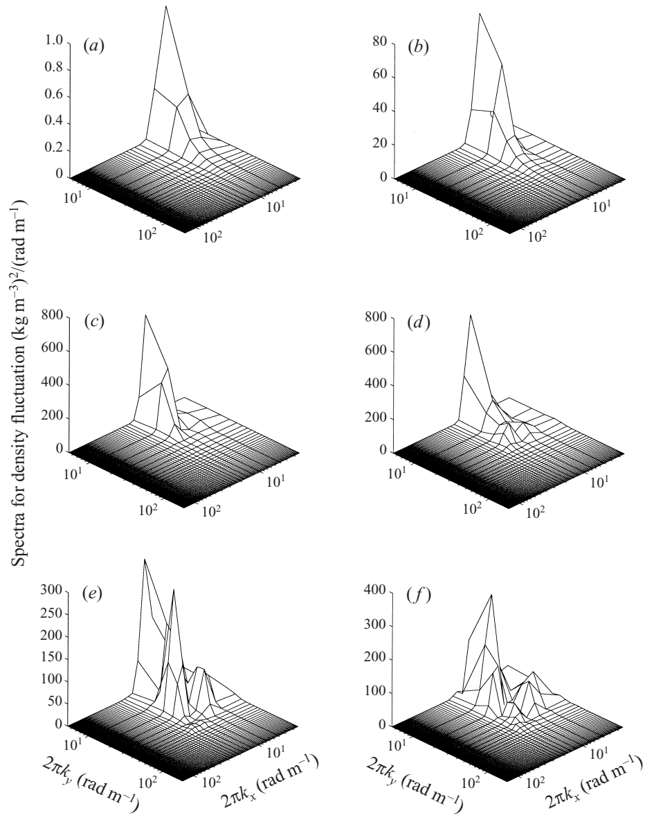
FIGURE 10. Two-dimensional wave number spectrum for the reflection region; Ke = 0.35 , Ri_m = 2.5 , Re = 23\,000 , and Pr = 7 . Times are (a) 2, (b) 4, (c) 8, (d) 10, (e) 11, and (f) 12. Higher wavenumbers appear as soon as the reflected and incident waves begin to interact spatially. For this case, the overturning occurs at T = 10.0 (figure 6).
