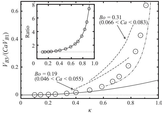
FIGURE 2. Migration velocity V_{B3} versus \kappa(=(1+\varepsilon)^{-1}) . The solid curve indicates the analytical solution (Magnaudet et al. 2003) V_{B3}/(CaV_{B1})=3\kappa^2(1+3\kappa/2)/\{40(1+3\kappa/4)\} with the assumption of the sufficiently long distance between the bubble centroid and the wall, i.e. \varepsilon \gg 1 . The dashed curves indicate the experimental results (Takemura et al. 2002), the circles the results obtained by the numerical simulation and the dash-dotted curve the prediction (2.24) by means of the lubrication approach (Hodges, Jensen & Rallison 2004). The inset shows the ratio of the simulation result to the analytical solution.
