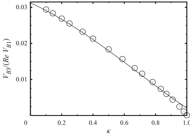
FIGURE 3. Inertia-driven migration velocity V_{B3} versus \kappa(=(1 + \varepsilon)^{-1}) for spherical bubble at 0 < Re \ll 1 . The solid curve indicates the analytical solution (Magnaudet et al. 2003) V_{B3}/(Re V_{B1}) = ((1 + \kappa/8 - 0.516\kappa^2)/32)(1 - (3/4)\kappa - (9/64)\kappa^4) under the assumption of (O(Re) < \kappa \ll 1) as in figure 2. The circles indicate the results obtained by the numerical simulation.
