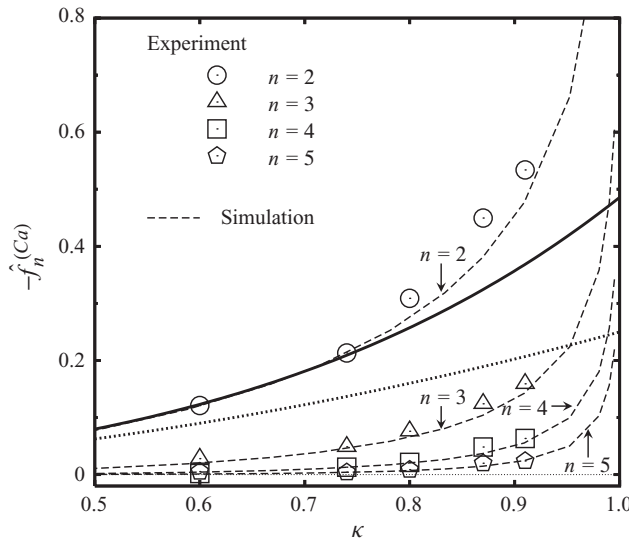
FIGURE 5. Modal deflection, \hat{f}_n^{(Ca)} , which is expanded in associated Legendre polynomials P_n^1 , versus \kappa(=(1 + \varepsilon)^{-1}) . The dotted curve indicates the leading term of the analytical solution (Magnaudet et al. 2003) \hat{f}_n^{(Ca)} = \kappa^2/4 and the solid curve indicates the analytical solution with the higher-order contributions \hat{f}_n^{(Ca)} = \kappa^2/4 \{1 + (3/8)\kappa (1 + (3/8)\kappa + (73/64)\kappa^2)\} . The symbols indicate the experimental results (Takemura et al. 2002) and the dashed curves indicate the results obtained by the numerical simulation.
