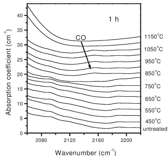
Figure 5. IR spectra of CO in the region 2060 – 2220\text{ cm}^{-1} in pyrophyllite EM08 samples (thin-sections) stepwise annealed for 1 h. Successive spectra have been offset vertically by 2\text{ cm}^{-1} for clarity.
