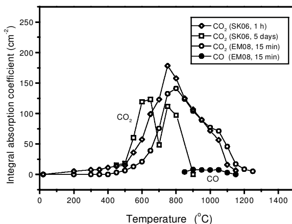
Figure 3. Temperature dependence of integral absorption coefficient (integral absorbance/sample thickness) of CO 2 (open symbols) and CO (filled circles) for different heating conditions (data from thin-sections).
