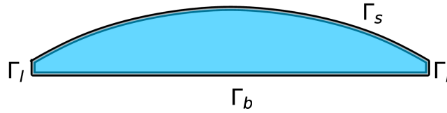
Fig. 1. A sketch representing the ice sheet boundary \partial\Omega subdivision into parts: \Gamma_l (the two lateral boundaries), \Gamma_s (the ice sheet free surface), and \Gamma_b (the ice sheet bedrock).
