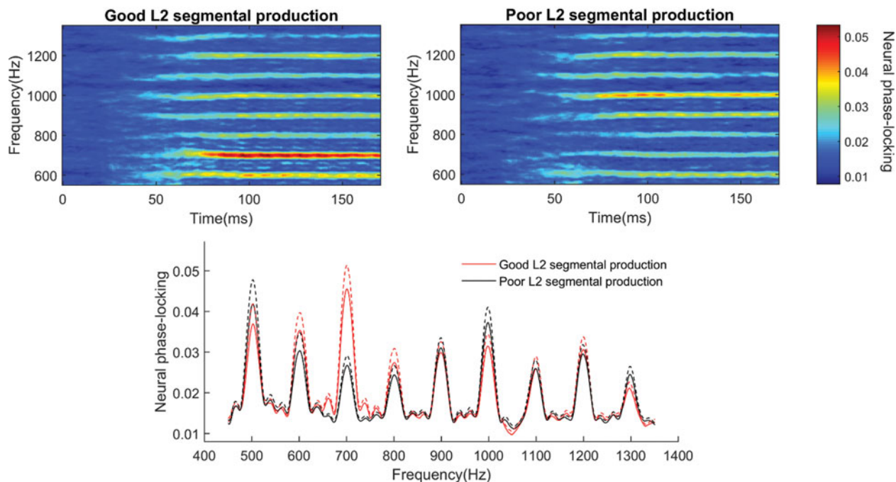
Figure 3. (Top) Inter-trial phase locking across time and frequency for participants with good (left) and poor (right) L2 segmental production scores (median split, n = 24 participants in each group). (Bottom) Inter-trial phase locking collapsed across time within a window from 60 to 170 ms in participants with good (red) and poor (black) L2 segmental production. Dotted lines indicate +1 standard error of the mean. Only the participants with good L2 segmental production showed a spectral peak around the first formant (700 Hz).
