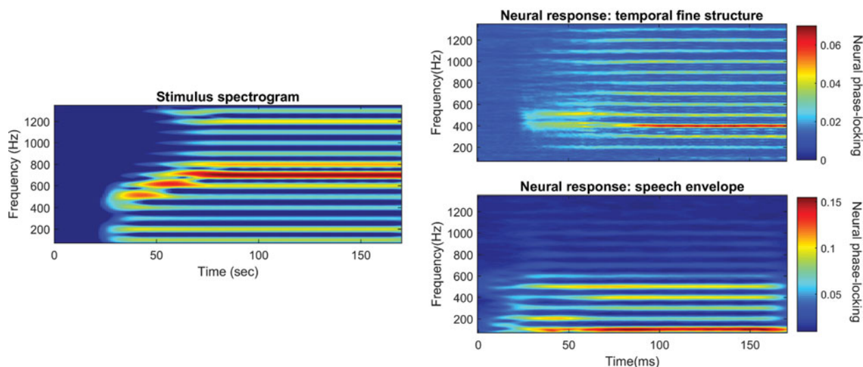
Figure 2. (Left) Spectrogram of stimulus used to evoke frequency-following responses. (Right) Inter-trial phase locking across time and frequency for the temporal fine structure response (top) and the envelope response (bottom).
