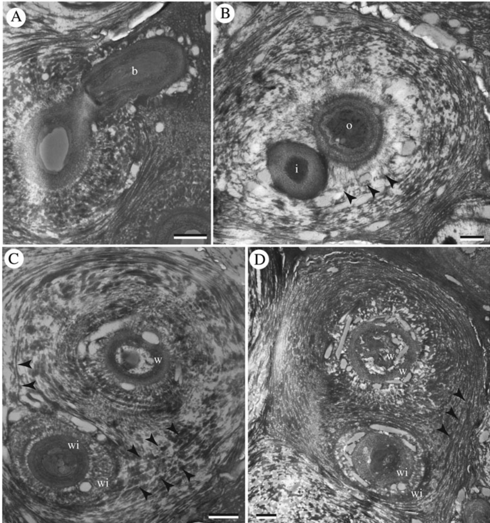
FIG. 5. TEM images of Ramalina usnea cortex, transverse section. Intrusive growth of branch filaments through the wall layers of neighbouring cells. A, branch filament (b) emerging in longitudinal view from cell in transverse orientation; B, younger filament (i) growing intrusively through wall materials produced by older cell (o). Note interruption of concentric layer of older cell's wall fragments (arrowheads) by younger intruding cell (i); C & D, walls of older cell (w) distinguished from those of younger intruding cell (wi) by their concentric orientation. Interruption of older neighbour's wall layers (arrowheads) by intruding filament. Scales: A–D = 500 nm.
