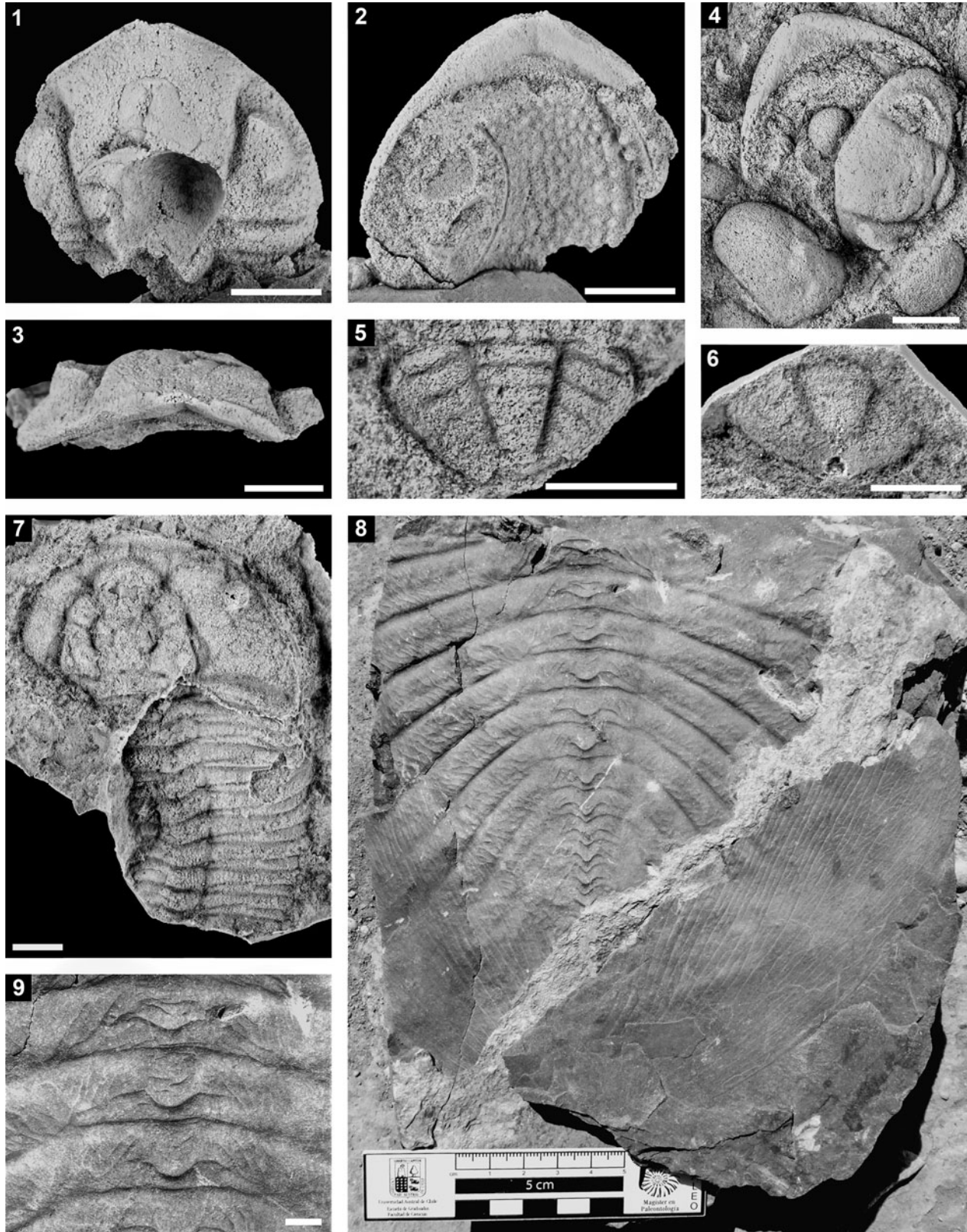
Figure 4. (1–6) Phacopidina quadrata (Hawle and Corda, 1847) from the Bofloss locality, Morocco. (1–3) Cephalon, internal mold, MGM-7681X: (1) dorsal view; (2) ventral view; (3) anterior view; (4) cephalon and cephalic doublure, internal molds, dorsal and ventral views, MGM-7689X-1 and 7689X-2, respectively; (5) pygidium, internal mold, MGM-7690X: dorsal view; (6) pygidium, latex cast of the external mold, MGM-7674X-3: dorsal view. (7) Prionocheilus cf. P. vermeilli Rouault, 1847, incomplete cephalon with thorax, latex cast of the external mold, MGM-7703X: dorsal view. (8, 9) Nobiliasaphus cf. N. kumatox Šnajdr, 1982a, pygidium, internal mold (field photograph): (8) dorsal view; (9) detail of the axis. All specimens are preserved in full relief (sandstones), except specimen (8, 9), preserved in mudstone. Scale bars = 5 mm.
