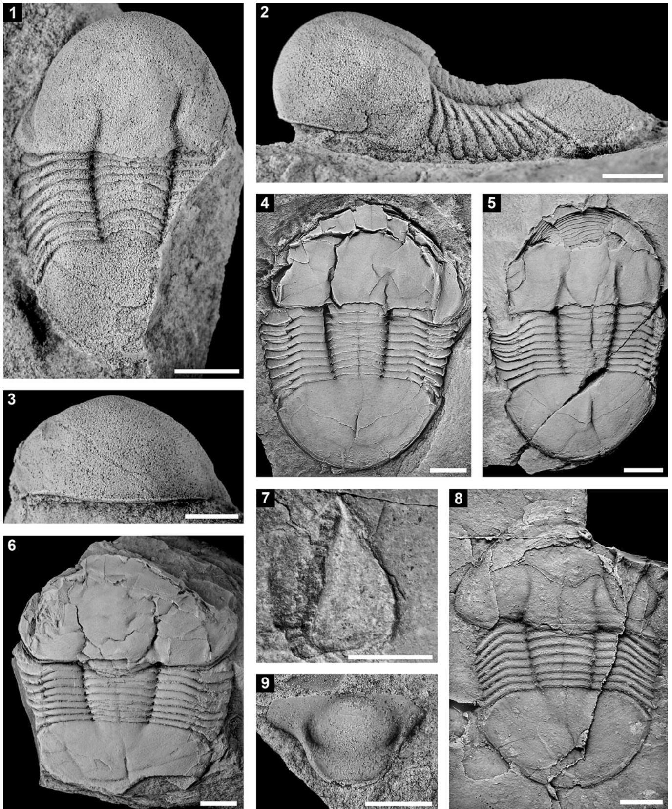
Figure 2. (1–8) Ulugtella? biformis n. sp., from the Bofloss locality, Morocco. (1–3) Exoskeleton, internal mold, holotype, MGM-7666X: (1) dorsal view; (2) left lateral view; (3) anterior view. (4) Exoskeleton, internal mold, paratype, MGM-7667X: dorsal view. (5) Exoskeleton, internal mold, paratype, MGM-7668X: dorsal view. (6) Exoskeleton, internal mold, paratype, MGM-7669X: dorsal view. (7, 8) Exoskeleton, paratype, MGM-7670X: (7) external mold of the left librigena; (8) latex cast of the external mold, MGM-7670X-1: dorsal view. (9) Hypostome, internal mold, paratype, MGM-7671X-1: ventral view. Specimens (1–3) and (9) are preserved in full relief (sandstones); the remaining specimens are preserved in mudstones, flattened. Scale bars = 5 mm.
