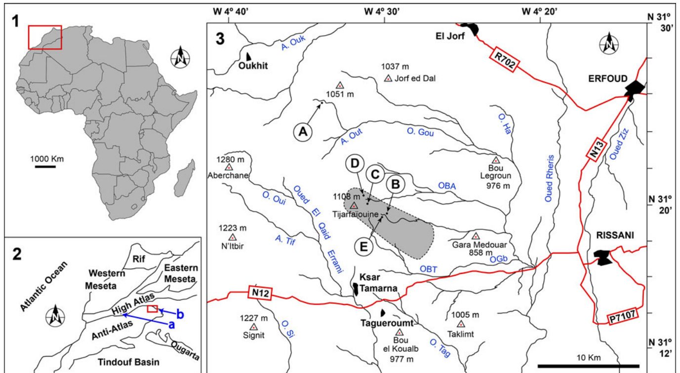
Figure 1. Sketch maps showing the position of the examined localities with reference to the African continent (1), the main Moroccan tectosedimentary basins (2), and a local map from the northwestern Tafilalet area, SE Morocco (3). Localities (a) and (b) in map (2) correspond to the early finds of the trilobite genus Declivolithus in the Skoura inlier of the central High Atlas (Destombes, 1971) and to the study area, respectively. The map (3) is a detail of the position of the fossiliferous localities mentioned in the text with reference to the road and drainage network, main populations, and geodesic vertices. The outline of Jbel Tijarfaiouine, the mountains where Declivolithus was first reported in the Eastern Anti-Atlas, is highlighted in gray. Fossil localities: (A) Bofloss; (B) Tifrit n'Ougnaou; (C) erroneous placement of the type locality of Declivolithus titan in the Jbel Tijarfaiouine according to Fortey and Edgecombe (2017); (D) Tizi n'Mouri; (E) erroneous placement of the Tifrit n'Ougnaou trilobite and echinoderm locality according to Lebrun (2018, p. 138). Abbreviations for other elements of the hydrological and drainage network: A. Oui = Assif n'Ouinigui; A. Ouk = Assif n'Oukhit; A. Out = Assif n'Outaouch; A. Tif = Assif Tifersiguet; OBA = Oued Bou Azgar; OBT = Oued Bou Terga; OGb = Oued Gbis; O. Gou = Oued Gounat; O. Ha = Oued Hanich; O. Si = Oued Signit; O. Tag = Oued Tagueroumt. Map and place names adapted from the sheets n° NH-30-XX-1, Misissi (published/edited in 1968) and NH-30-XX-2, Erfoud (published/edited in 1970) of the Topographic Map of Morocco at a scale of 1:100,000.
