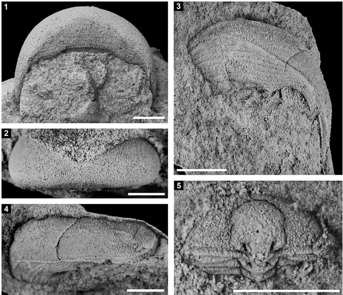
Figure 9. (1–4) Symphysops stevaninae Lopéz-Soriano and Corbacho, 2012, from the Bofloss locality, Morocco. (1, 2) Visual surface and cephalic doublure, internal mold, MGM-7737X: (1) ventral view; (2) anterior view; (3, 4) visual surface and cephalic doublure, latex cast of the external mold, MGM-7738X: (3) oblique ventral view; (4) oblique left anteroventral view. (5) Dionide sp. from the Bofloss locality, Morocco. Incomplete cephalon with thorax, internal mold, MGM-7671X-2: dorsal view. All specimens preserved in full relief (sandstones). Scale bars = 5 mm.
