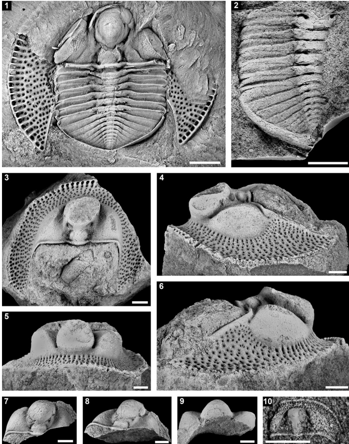
Figure 11. (1–10) Declivolithus alfredi (Želízko, 1906) from the Bofloss locality, Morocco. (1) Exoskeleton, latex cast of the external mold, MGM-7745X: dorsal view; (2) incomplete thorax with pygidium, latex cast of the external mold, MGM-7765X: dorsal view; (3–6) cephalon, internal mold (lower lamella missing), MGM-7749X: (3) dorsal view; (4) left lateral view; (5) anterior view; (6) right lateral view; (7–9) cephalon (fringe missing), internal mold, MGM-7750X: (7) dorsal view; (8) oblique right posterolateral view; (9) anterior view; (10) meraspis cephalon, latex cast of the external mold, MGM-7771X: dorsal view. All specimens are preserved in full relief (sandstones), except specimen (1), preserved in mudstone, flattened. Scale bars = 5 mm, except (10) = 2 mm.
