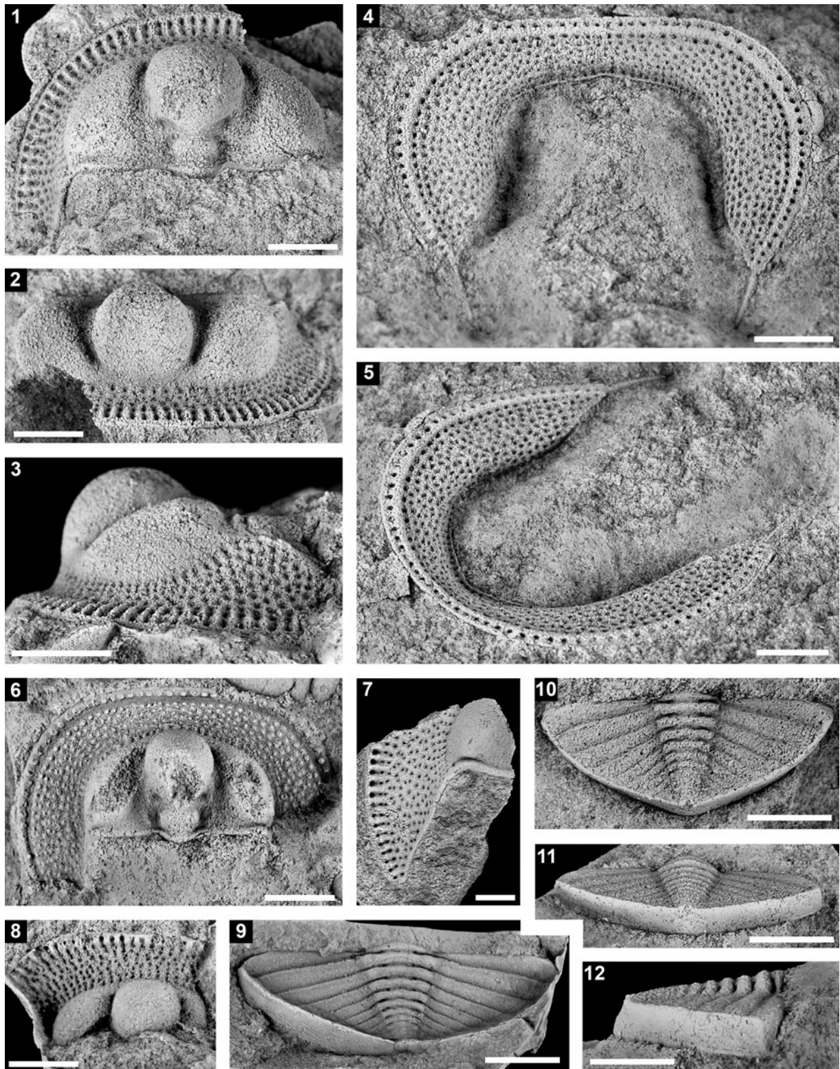
Figure 12. (1–12) Declivolithus alfredi (Želízko, 1906) from the Bofloss locality, Morocco. (1–3) Cephalon, internal mold, MGM-7751X: (1) dorsal view; (2) anterodorsal view; (3) left lateral view; (4, 5) lower lamella of the fringe, internal mold, MGM-7761X: (4) ventral view; (5) oblique right ventrolateral view; (6) cephalon (upper lamella missing), internal mold, MGM-7752X: dorsal view; (7) incomplete cephalon (left genal lobe and posterior left part of the fringe), internal mold, MGM-7753X: dorsal view; (8) incomplete cephalon, latex cast of the external mold, MGM-7754X: anterodorsal view; (9) pygidium, latex cast of the external mold, MGM-7768X: dorsoposterior view. (10–12) Pygidium, internal mold, MGM-7767X-1: (10) dorsal view; (11) posterior view; (12) right lateral view. All specimens are preserved in full relief (sandstones), except specimen (9), preserved in mudstone, flattened. Scale bars = 5 mm.
