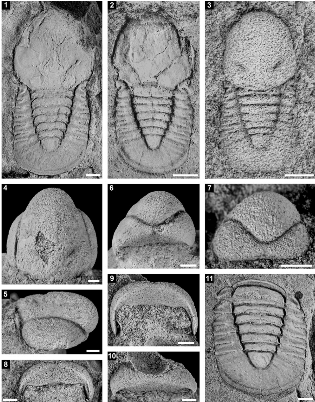
Figure 7. (1–11) Cyclopyge cf. C. rediviva (Barrande, 1846) from the Bofloss locality, Morocco. (1) Exoskeleton, internal mold, MGM-7708X: dorsal view; (2) exoskeleton, internal mold, MGM-7709X: dorsal view; (3) exoskeleton, latex cast of the external mold, MGM-7710Xa: dorsal view; (4–6) cephalon, internal mold, MGM-7711X: (4) dorsal view; (5) right lateral view; (6) anterior view; (7) cephalon, internal mold, MGM-7712X-1: anterior view; (8) visual surface and cephalic doublure, internal mold, MGM-7712X-2: anteroventral view; (9, 10) visual surface and cephalic doublure, internal mold, MGM-7713X: (9) anteroventral view; (10) anterior view; (11) thorax with pygidium, internal mold, MGM-7714X: dorsal view. Specimens (1–2) and (11) are preserved in mudstones, flattened; the remaining are preserved in full relief (sandstones). Scale bars = 2 mm.
