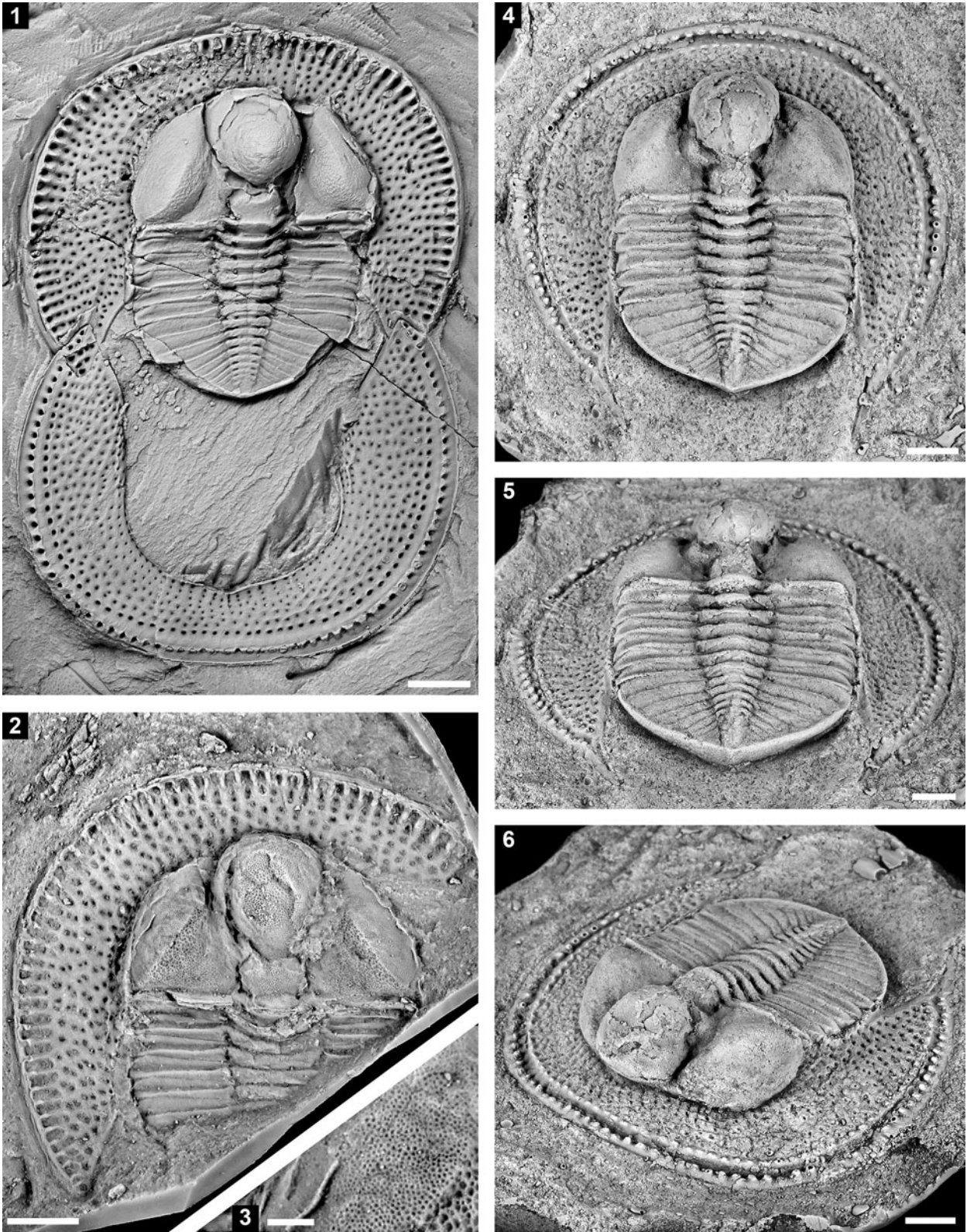
Figure 10. (1–6) Declivolithus alfredi (Želízko, 1906) from the Bofloss locality, Morocco. (1) Exoskeleton (molting configuration), internal mold, MGM-7742X: dorsal and ventral (lower lamella) views; (2, 3) incomplete cephalon with thorax, latex cast of the external mold, MGM-7743X: (2) dorsal view; (3) detail of the external sculpture of the left genal lobe; (4–6) exoskeleton (upper lamella missing), dental plaster replica of the internal mold, MGM-7744X-R: (4) dorsal view; (5) dorsoposterior view; (6) oblique left anterolateral view. Specimens (1, 2) are preserved in mudstones, flattened; specimen (4–6) preserved in full relief (sandstone). Scale bars = 5 mm.
