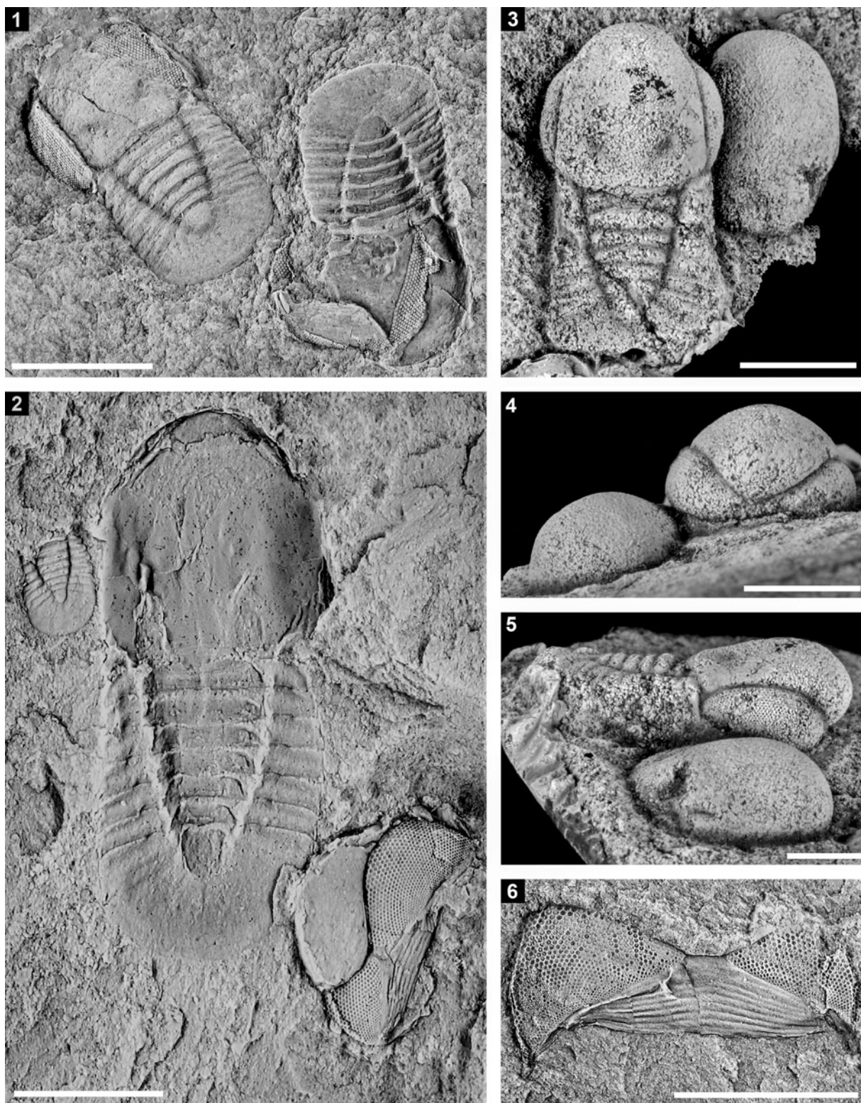
Figure 6. (1–6) Cyclopyge cf. C. rediviva (Barrande, 1846) from the Bofloss locality, Morocco. (1) Two exoskeletons, latex cast of internal (MGM-7704X-1a, left) and external (MGM-7704X-2a, right) molds: dorsal view, showing traces of the visual surfaces; (2) exoskeleton (center), meraspis thorax with pygidium (upper left) and cephalon (lower right), internal and external molds, MGM-7705X-1, MGM-7705X-3, and MGM-7705X-2, respectively: dorsal and anterior views; (3–5) exoskeleton, internal mold, MGM-7706X: (3) dorsal view; (4) anterior view; (5) right lateral view; (6) visual surface and cephalic doublure, latex cast of the external mold, MGM-7707Xa: anteroventral view. Specimens (3–5) are preserved in full relief (sandstones); the remaining specimens are preserved in mudstones, flattened. Scale bars = 5 mm.
