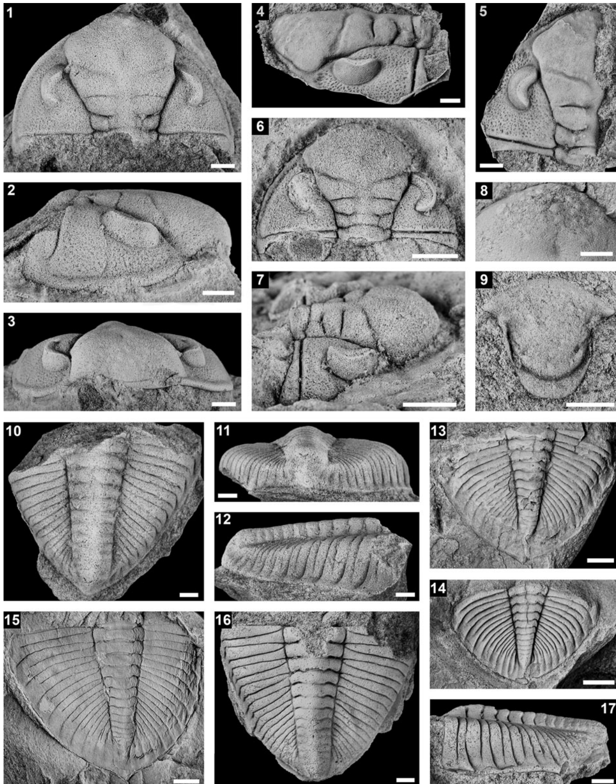
Figure 5. (1–17) Eudolaites cf. E. bondoni Destombes, 1972, from the Bofloss locality, Morocco. (1–3) Cephalon, internal mold, MGM-7692X: (1) dorsal view; (2) right lateral view; (3) anterior view; (4, 5) incomplete cephalon, latex cast of the external mold, MGM-7696X-1: (4) left lateral view; (5) dorsal view; (6, 7) cephalon, internal mold, MGM-7693X: (6) dorsal view; (7) right lateral view; (8) cephalon, internal mold, MGM-7694X: detail of the frontal lobe showing auxiliary impressions; (9) hypostome, internal mold, MGM-7702X: ventral view; (10–12) pygidium, internal mold, MGM-7697X: (10) dorsal view; (11) posterior view; (12) right lateral view; (13) pygidium, internal mold, MGM-7699X: dorsal view; (14) pygidium, internal mold, MGM-7700X: dorsal view; (15) pygidium, latex cast of the external mold, MGM-7701X: dorsal view; (16, 17) pygidium, internal mold, MGM-7696X-2: (16) dorsal view; (17) left lateral view. All specimens are preserved in full relief (sandstones), except specimens (13–15), which are preserved in mudstones (flattened). Scale bars = 5 mm.
