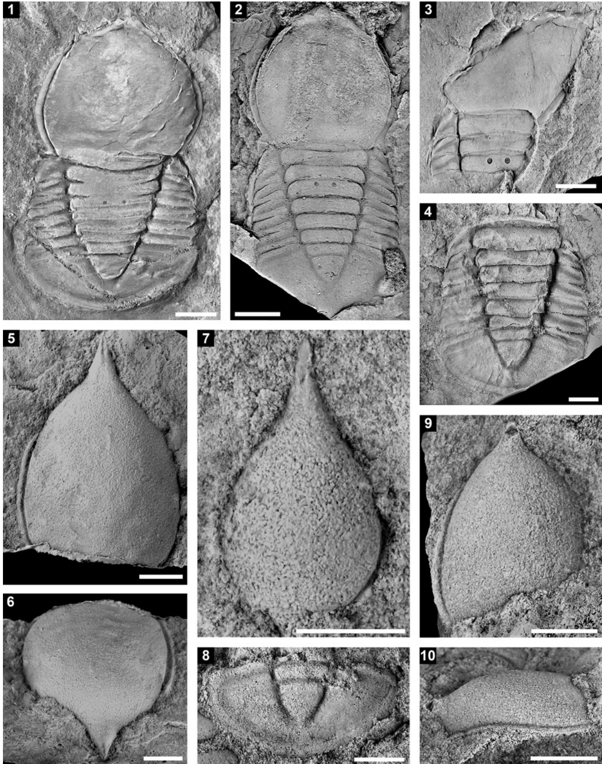
Figure 8. (1–10) Symphysops stevaninae López-Soriano and Corbacho, 2012, from the Bofloss locality, Morocco. (1) Exoskeleton, internal mold, MGM-7731X: dorsal view; (2) exoskeleton, latex cast of the external mold, MGM-7732X: dorsal view; (3) incomplete cephalon with thorax, internal mold, MGM-7739X: dorsal view; (4) thorax with pygidium, latex cast of the external mold, MGM-7691X: dorsal view; (5, 6) cranium, latex cast of the external mold, MGM-7733X: (5) dorsal view; (6) anterior view; (7) cranium, internal mold, MGM-7734X: dorsal view; (8) pygidium, internal mold, MGM-7740X: dorsal view; (9, 10) cranium, internal mold, MGM-7735X: (9) dorsal view; (10) left lateral view. Specimens (1–4) are preserved in mudstones, flattened; the remaining specimens are preserved in full relief (sandstones). Scale bars = 5 mm.
