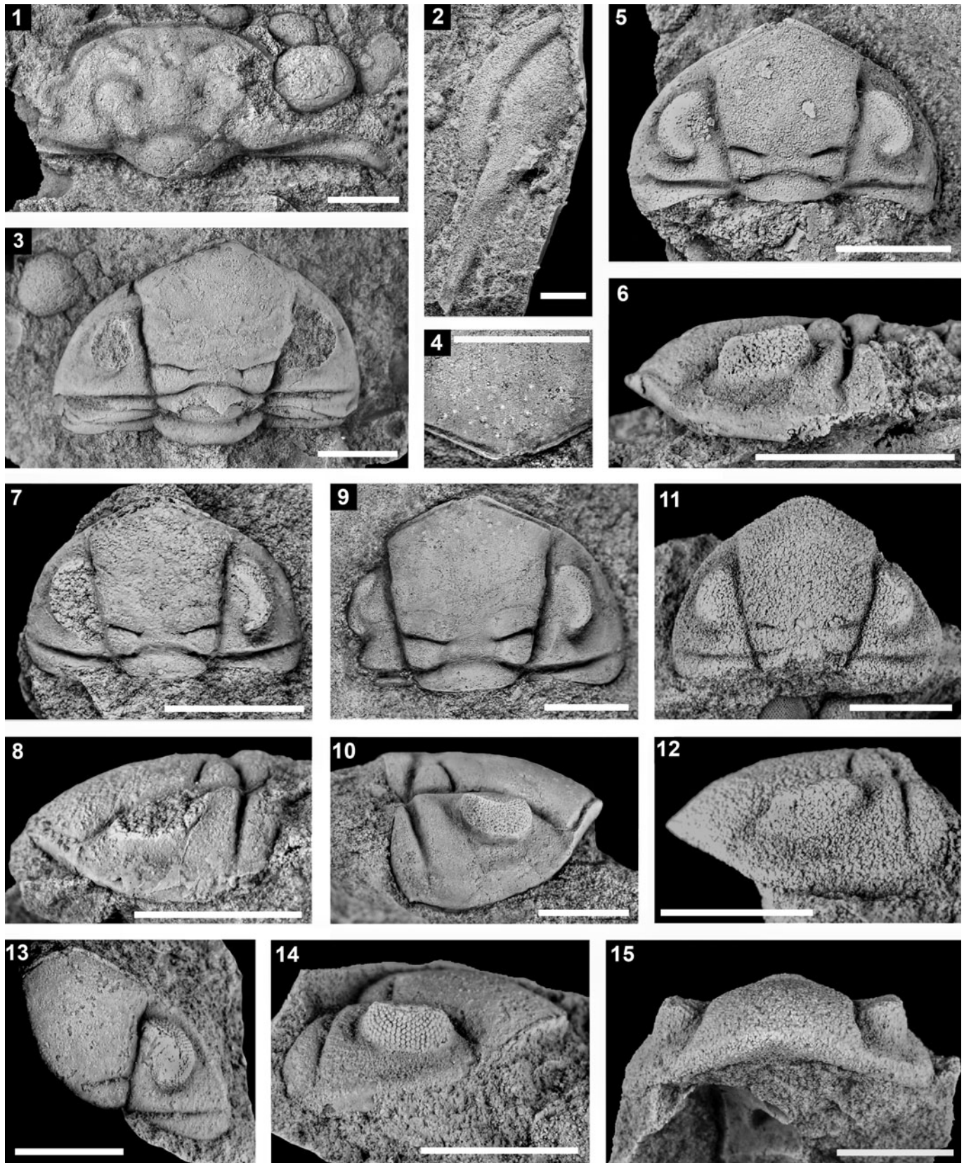
Figure 3. (1, 2) Selenopeltis cf. S. vultuosa Přibyl and Vaněk, 1966, from the Bofloss locality, Morocco. (1) Cranidium, internal mold, MGM-7673X: dorsal view; (2) left librigena, latex cast of the external mold, MGM-7674X-1. (3–15) Phacopidina quadrata (Hawle and Corda, 1847) from the Bofloss locality, Morocco. (3) Cephalon, internal mold, MGM-7675X: dorsal view; (4, 9, 10) cephalon, internal mold, MGM-7676X: (4) frontal view showing frontal lobe auxiliary impressions; (9) dorsal view; (10) right lateral view; (5, 6) cephalon, internal mold, MGM-7677X: (5) dorsal view; (6) left lateral view; (7, 8) cephalon, internal mold, MGM-7678X: (7) dorsal view; (8) left lateral view; (11, 12, 15) cephalon, internal mold, MGM-7679X: (11) dorsal view; (12) left lateral view; (15) anterior view; (13, 14) cephalon, latex cast of the external mold, MGM-7680X: (13) dorsal view; (14) right lateral view. All specimens are preserved in full relief (sandstones). Scale bars = 5 mm.
