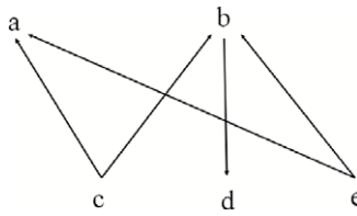
Fig. 2. Dependency graph DG(\Pi) .
