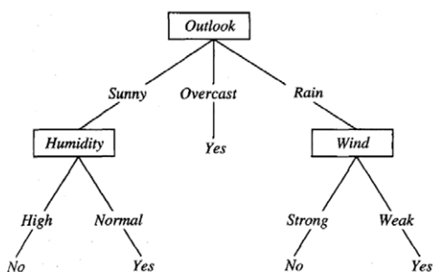
Fig. 1. A decision tree.
