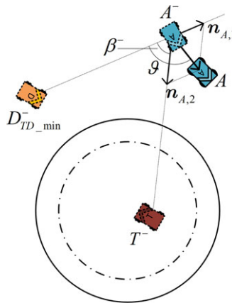
Figure 5. Intention prediction of the attacker.
