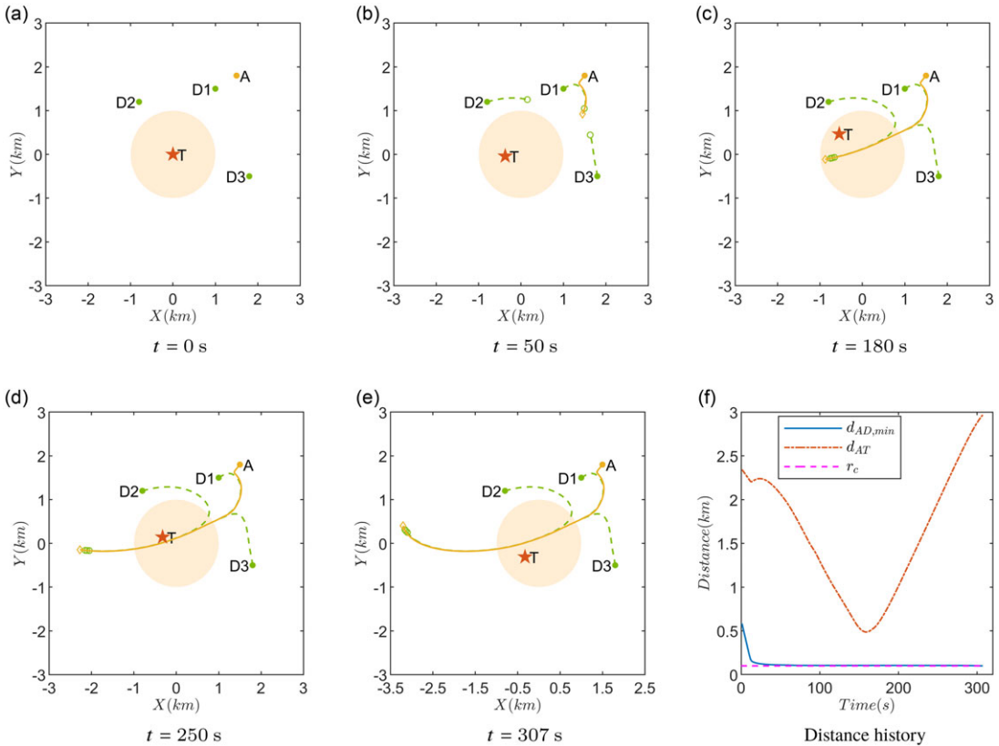
Figure 11. Simulation results of pure pursuit strategy.
