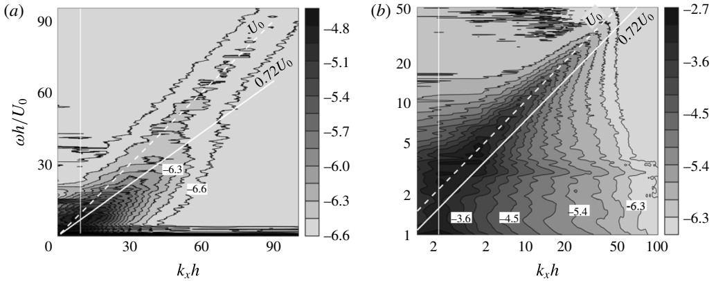
FIGURE 12. The measured wavenumber–frequency spectra of detrended deformation, with contours indicating the values of \log_{10}\{E_{dd}(k_x, \omega)U_0/[h(\rho u_\tau^2 l_0/E')]^2\} . (a) Small field-of-view data on linear axes, with an incremental increase between contour lines of 0.15. (b) Large field-of-view data on logarithmic axes, with an incremental increase between contour lines of 0.3. The inclined solid and dashed lines represent advection speeds of 0.72U_0 and U_0 , respectively. The vertical lines in each figure show the wavenumber of the corresponding field of view.
