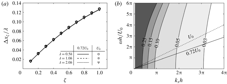
FIGURE 16. The streamwise offset between deformation and pressure correlation peak predicted by the Chase (1991) model: (a) values of \Delta x_\zeta/\lambda for pressure perturbations with the specified wavelengths and advection speeds, and (b) values of \Delta x_\zeta/h as functions of wavenumber and frequency for \zeta = 0.3 .
