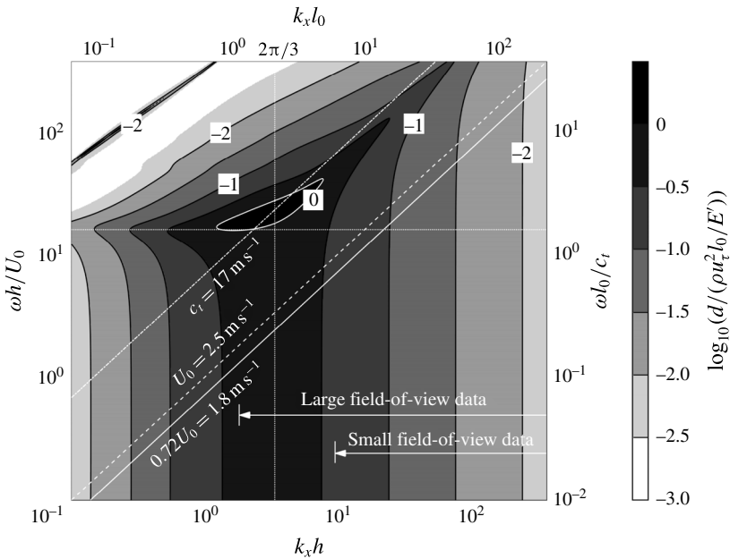
FIGURE 11. The amplitude of deformation (normalized by \rho u_t^2 l_0 / E' ) in response to pressure perturbation amplitude of \rho u_t^2 , as predicted by the Chase (1991) model. The inclined lines correspond to the specified advection speeds. The vertical and horizontal dotted lines represent k_x l_0 = 2\pi/3 and \omega l_0 / c_t = 1.45 , respectively.
